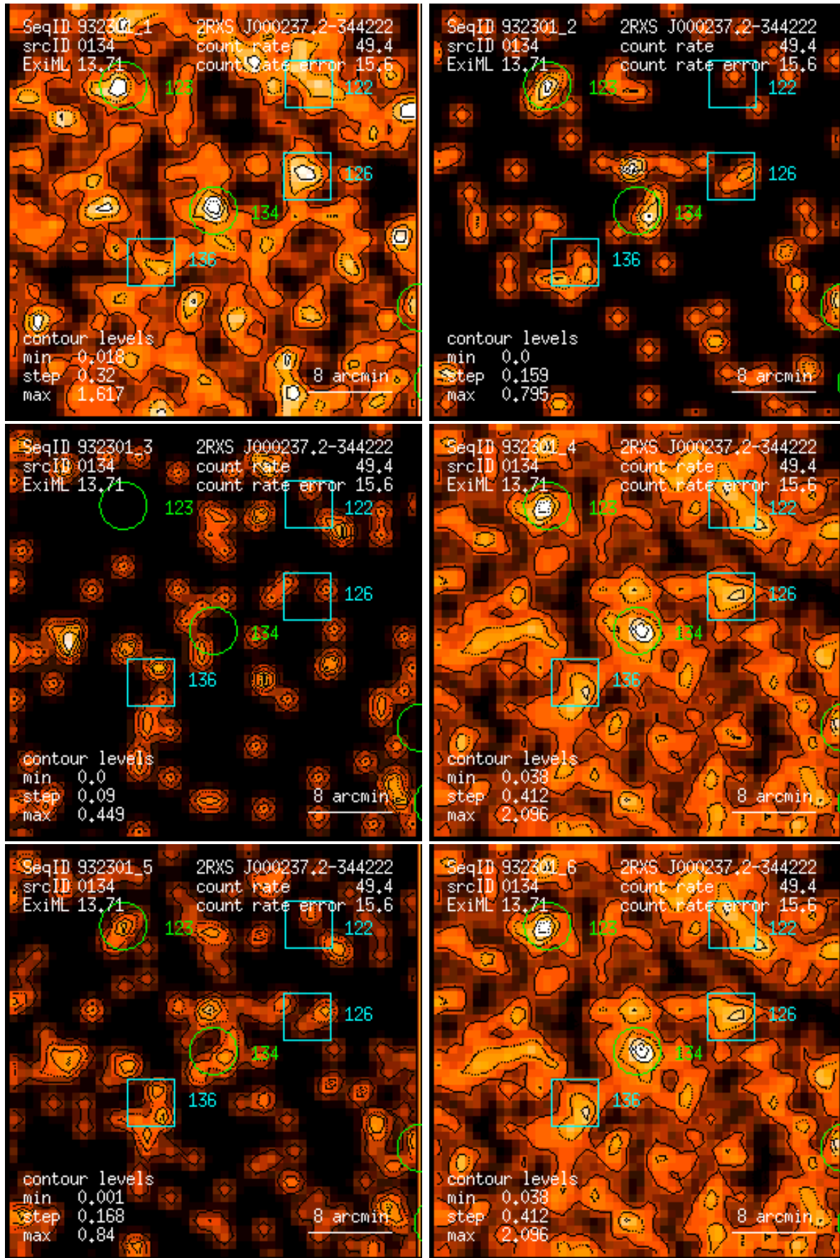
Figure 134: RASS 932301: detection 0134: band rate images, Gaussian filter: (1) PSPC channels 11 – 41, (2) 52 – 90, (3) 91 – 201, (4) 11 – 235, (5) 52 – 201, (6) 11 – 201. Broad band rates in counts/ks. Band rate contour levels in counts/ks/arcmin 2 .
