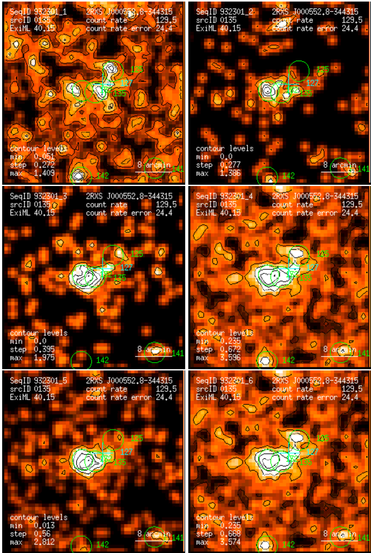
Figure 135: RASS 932301: detection 0135: band rate images, Gaussian filter: (1) PSPC channels 11 – 41, (2) 52 – 90, (3) 91 – 201, (4) 11 – 235, (5) 52 – 201, (6) 11 – 201. Broad band rates in counts/ks. Band rate contour levels in counts/ks/arcmin 2 .
