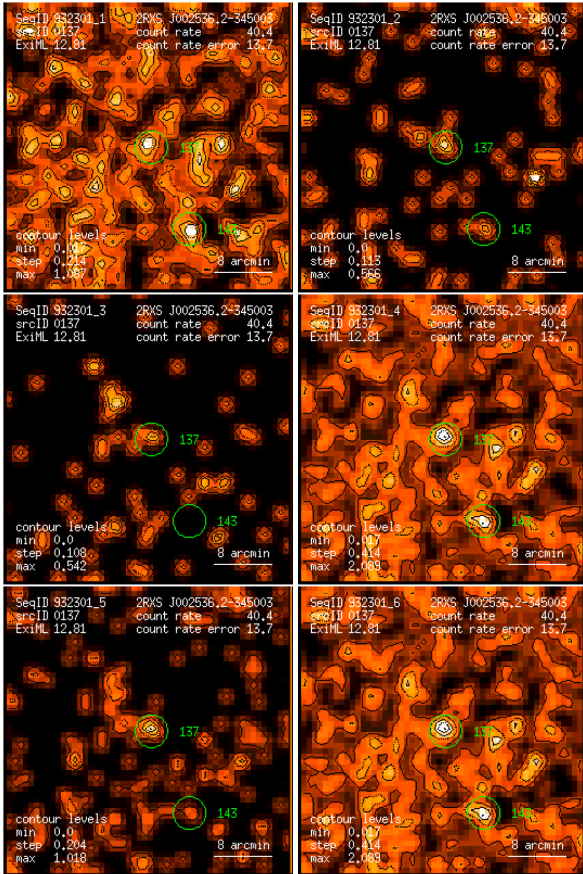
Figure 137: RASS 932301: detection 0137: band rate images, Gaussian filter: (1) PSPC channels 11 – 41, (2) 52 – 90, (3) 91 – 201, (4) 11 – 235, (5) 52 – 201, (6) 11 – 201. Broad band rates in counts/ks. Band rate contour levels in counts/ks/arcmin 2 .
