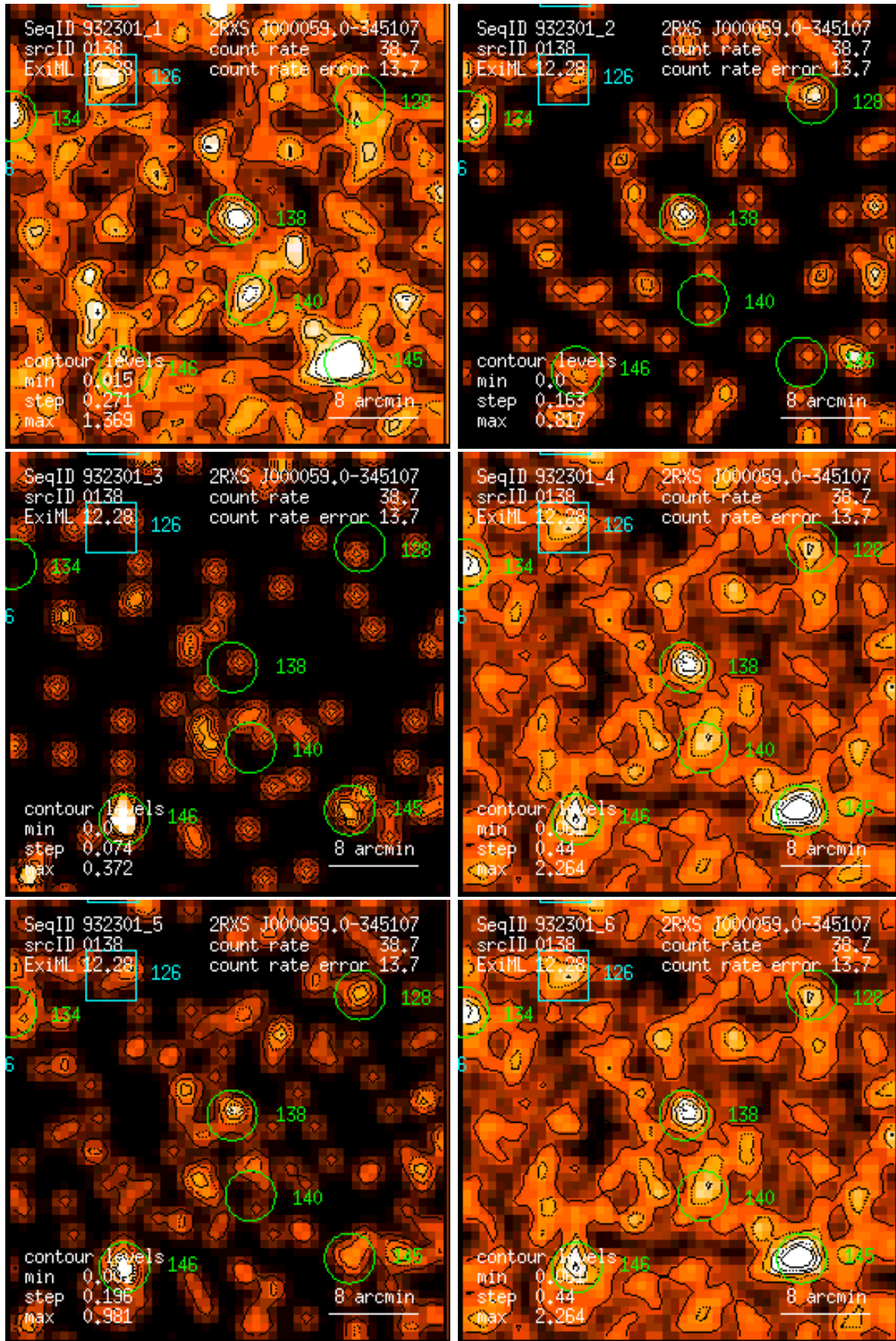
Figure 138: RASS 932301: detection 0138: band rate images, Gaussian filter: (1) PSPC channels 11 – 41, (2) 52 – 90, (3) 91 – 201, (4) 11 – 235, (5) 52 – 201, (6) 11 – 201. Broad band rates in counts/ks. Band rate contour levels in counts/ks/arcmin 2 .
