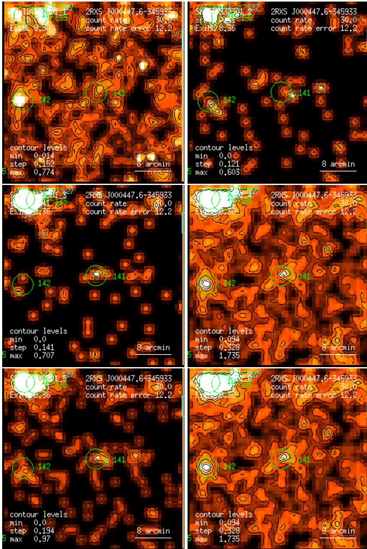
Figure 141: RASS 932301: detection 0141: band rate images, Gaussian filter: (1) PSPC channels 11 – 41, (2) 52 – 90, (3) 91 – 201, (4) 11 – 235, (5) 52 – 201, (6) 11 – 201. Broad band rates in counts/ks. Band rate contour levels in counts/ks/arcmin 2 .
