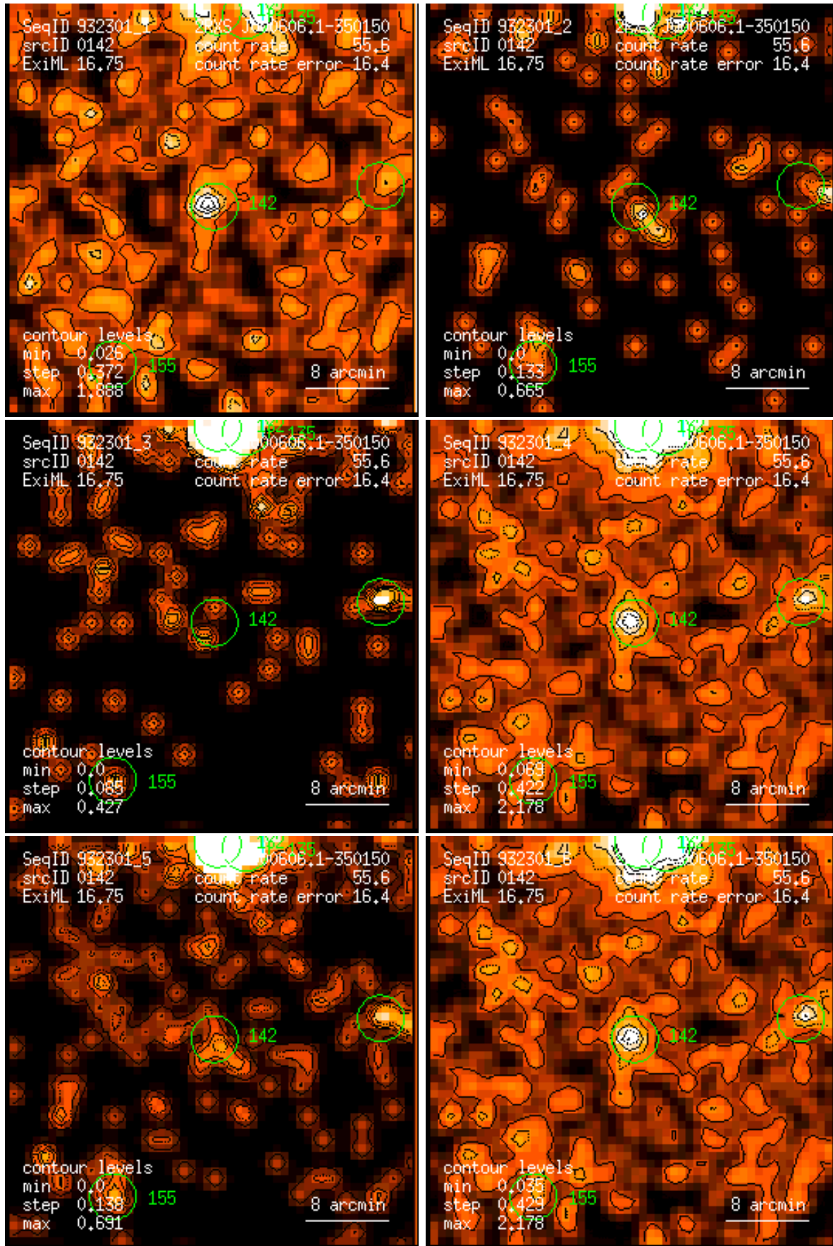
Figure 142: RASS 932301: detection 0142: band rate images, Gaussian filter: (1) PSPC channels 11 – 41, (2) 52 – 90, (3) 91 – 201, (4) 11 – 235, (5) 52 – 201, (6) 11 – 201. Broad band rates in counts/ks. Band rate contour levels in counts/ks/arcmin 2 .
