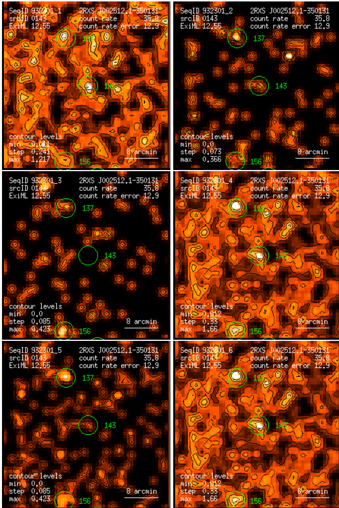
Figure 143: RASS 932301: detection 0143: band rate images, Gaussian filter: (1) PSPC channels 11 – 41, (2) 52 – 90, (3) 91 – 201, (4) 11 – 235, (5) 52 – 201, (6) 11 – 201. Broad band rates in counts/ks. Band rate contour levels in counts/ks/arcmin 2 .
