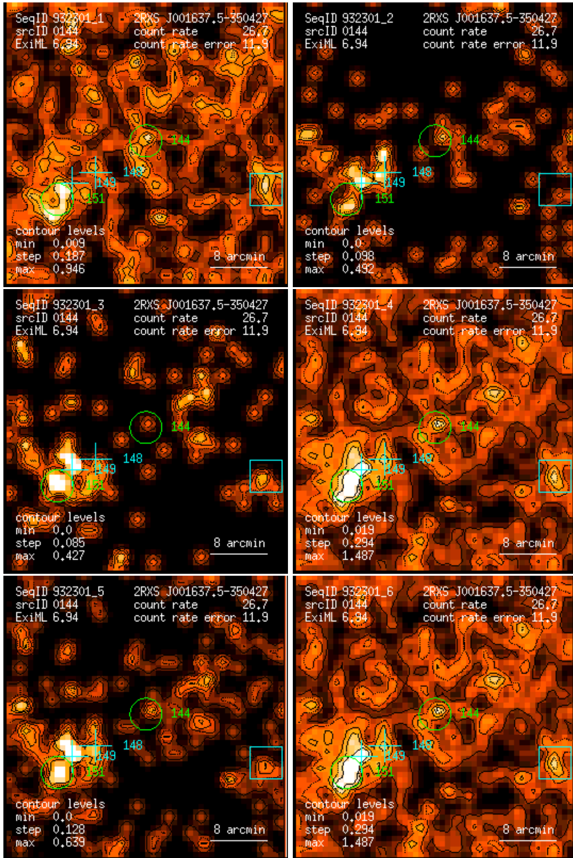
Figure 144: RASS 932301: detection 0144: band rate images, Gaussian filter: (1) PSPC channels 11 – 41, (2) 52 – 90, (3) 91 – 201, (4) 11 – 235, (5) 52 – 201, (6) 11 – 201. Broad band rates in counts/ks. Band rate contour levels in counts/ks/arcmin 2 .
