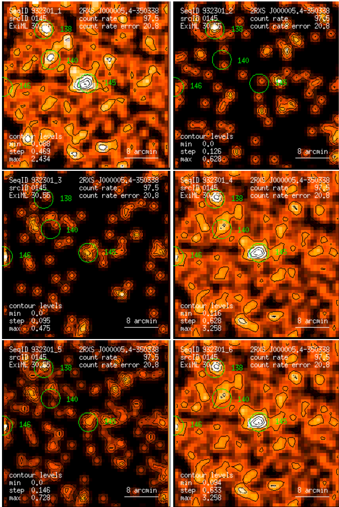
Figure 145: RASS 932301: detection 0145: band rate images, Gaussian filter: (1) PSPC channels 11 – 41, (2) 52 – 90, (3) 91 – 201, (4) 11 – 235, (5) 52 – 201, (6) 11 – 201. Broad band rates in counts/ks. Band rate contour levels in counts/ks/arcmin 2 .
