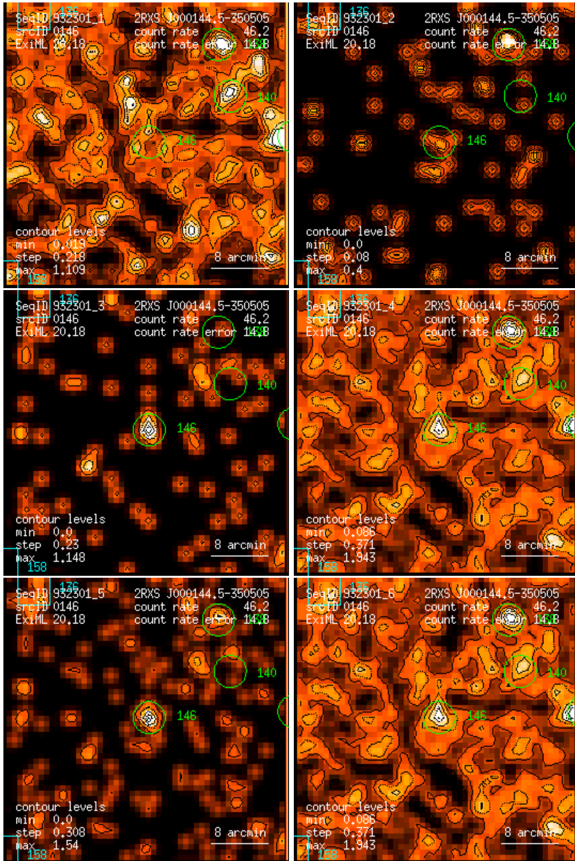
Figure 146: RASS 932301: detection 0146: band rate images, Gaussian filter: (1) PSPC channels 11 – 41, (2) 52 – 90, (3) 91 – 201, (4) 11 – 235, (5) 52 – 201, (6) 11 – 201. Broad band rates in counts/ks. Band rate contour levels in counts/ks/arcmin 2 .
