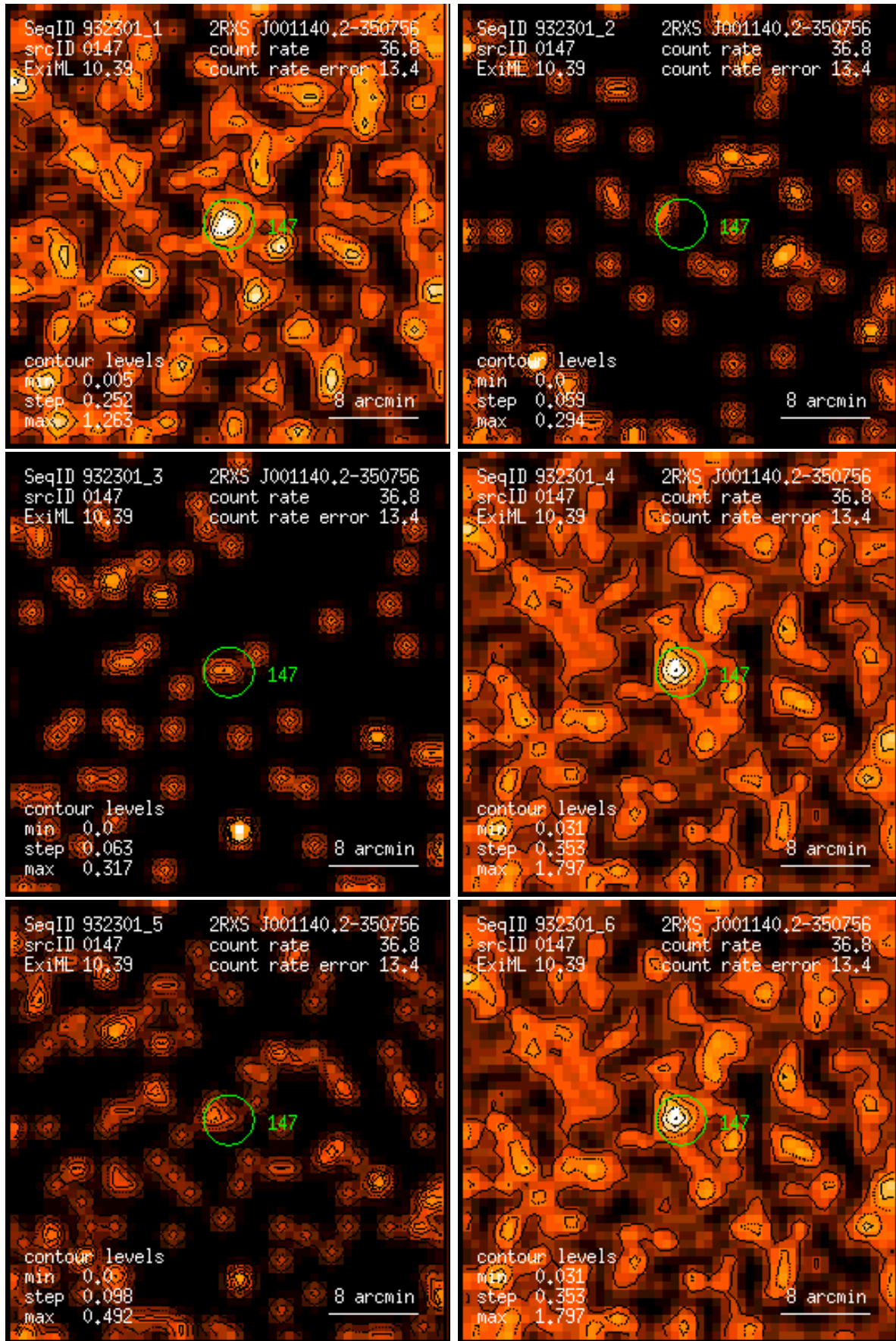
Figure 147: RASS 932301: detection 0147: band rate images, Gaussian filter: (1) PSPC channels 11 – 41, (2) 52 – 90, (3) 91 – 201, (4) 11 – 235, (5) 52 – 201, (6) 11 – 201. Broad band rates in counts/ks. Band rate contour levels in counts/ks/arcmin 2 .
