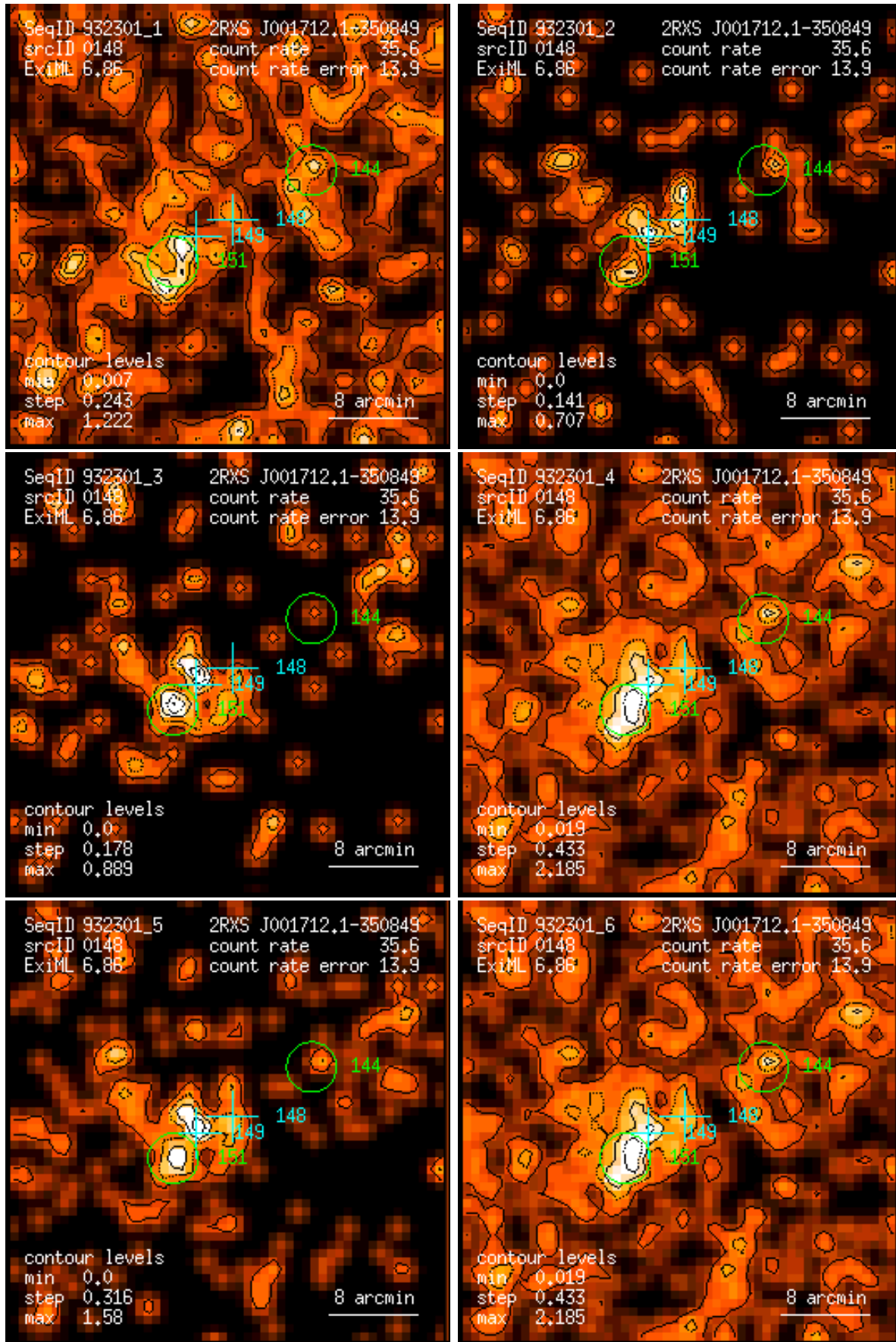
Figure 148: RASS 932301: detection 0148: band rate images, Gaussian filter: (1) PSPC channels 11 – 41, (2) 52 – 90, (3) 91 – 201, (4) 11 – 235, (5) 52 – 201, (6) 11 – 201. Broad band rates in counts/ks. Band rate contour levels in counts/ks/arcmin 2 .
