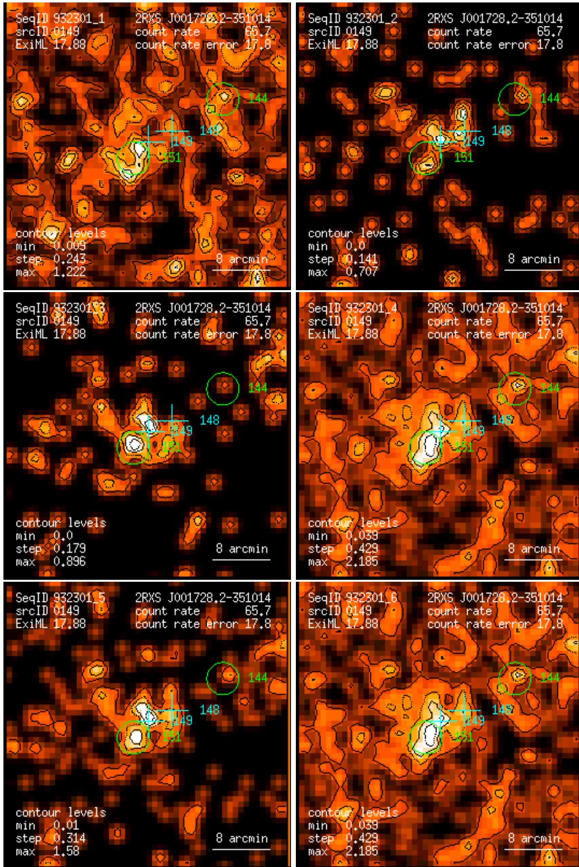
Figure 149: RASS 932301: detection 0149: band rate images, Gaussian filter: (1) PSPC channels 11 – 41, (2) 52 – 90, (3) 91 – 201, (4) 11 – 235, (5) 52 – 201, (6) 11 – 201. Broad band rates in counts/ks. Band rate contour levels in counts/ks/arcmin 2 .
