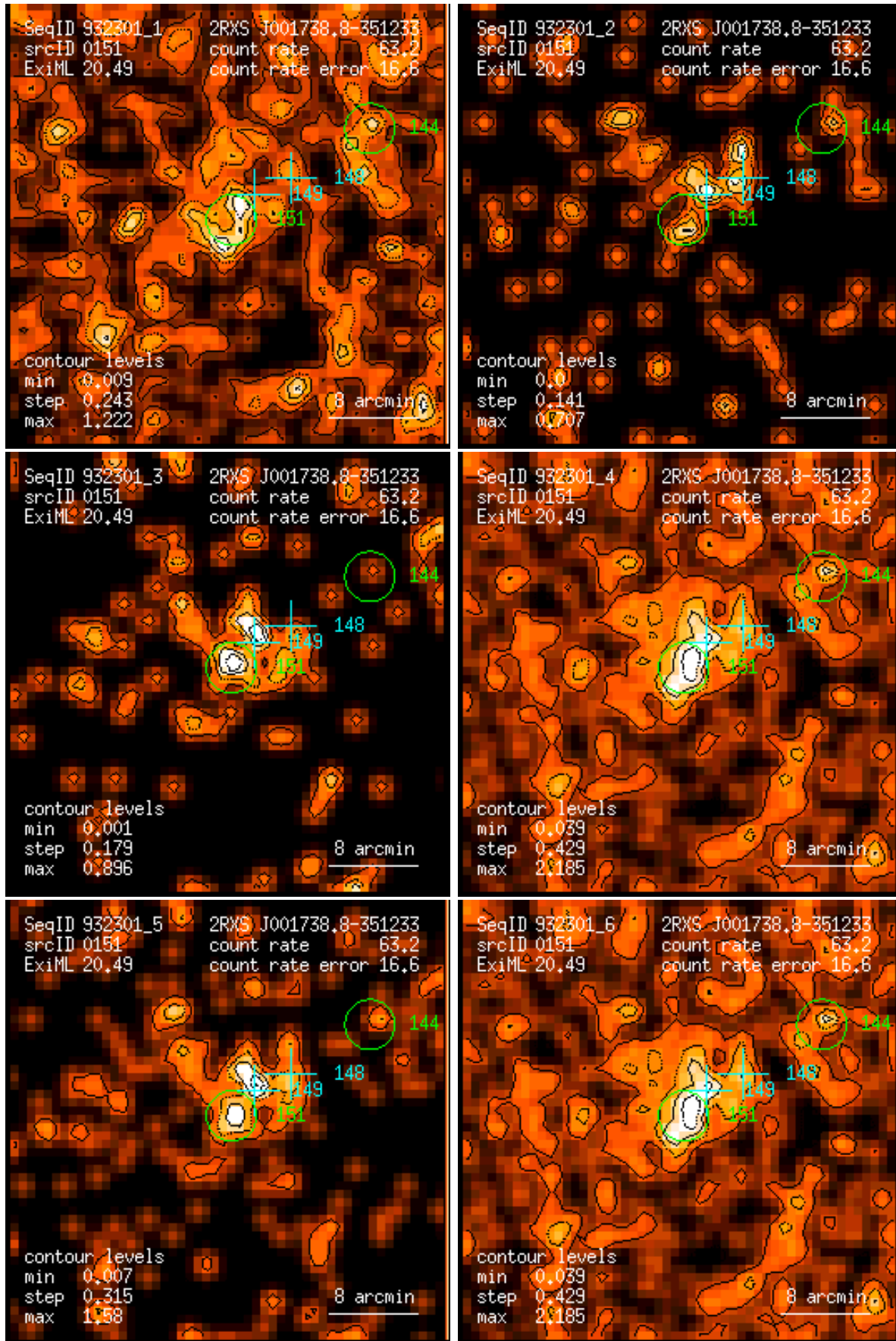
Figure 151: RASS 932301: detection 0151: band rate images, Gaussian filter: (1) PSPC channels 11 – 41, (2) 52 – 90, (3) 91 – 201, (4) 11 – 235, (5) 52 – 201, (6) 11 – 201. Broad band rates in counts/ks. Band rate contour levels in counts/ks/arcmin 2 .
