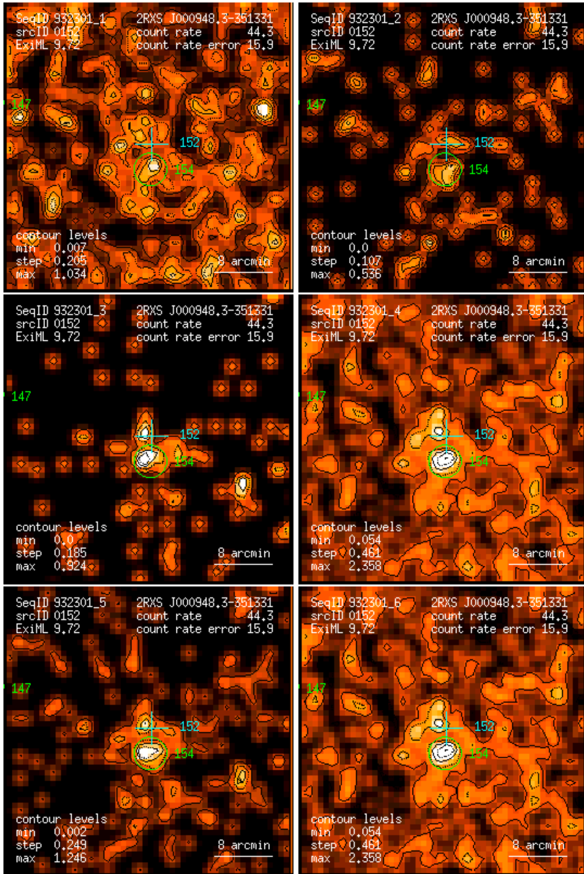
Figure 152: RASS 932301: detection 0152: band rate images, Gaussian filter: (1) PSPC channels 11 – 41, (2) 52 – 90, (3) 91 – 201, (4) 11 – 235, (5) 52 – 201, (6) 11 – 201. Broad band rates in counts/ks. Band rate contour levels in counts/ks/arcmin 2 .
