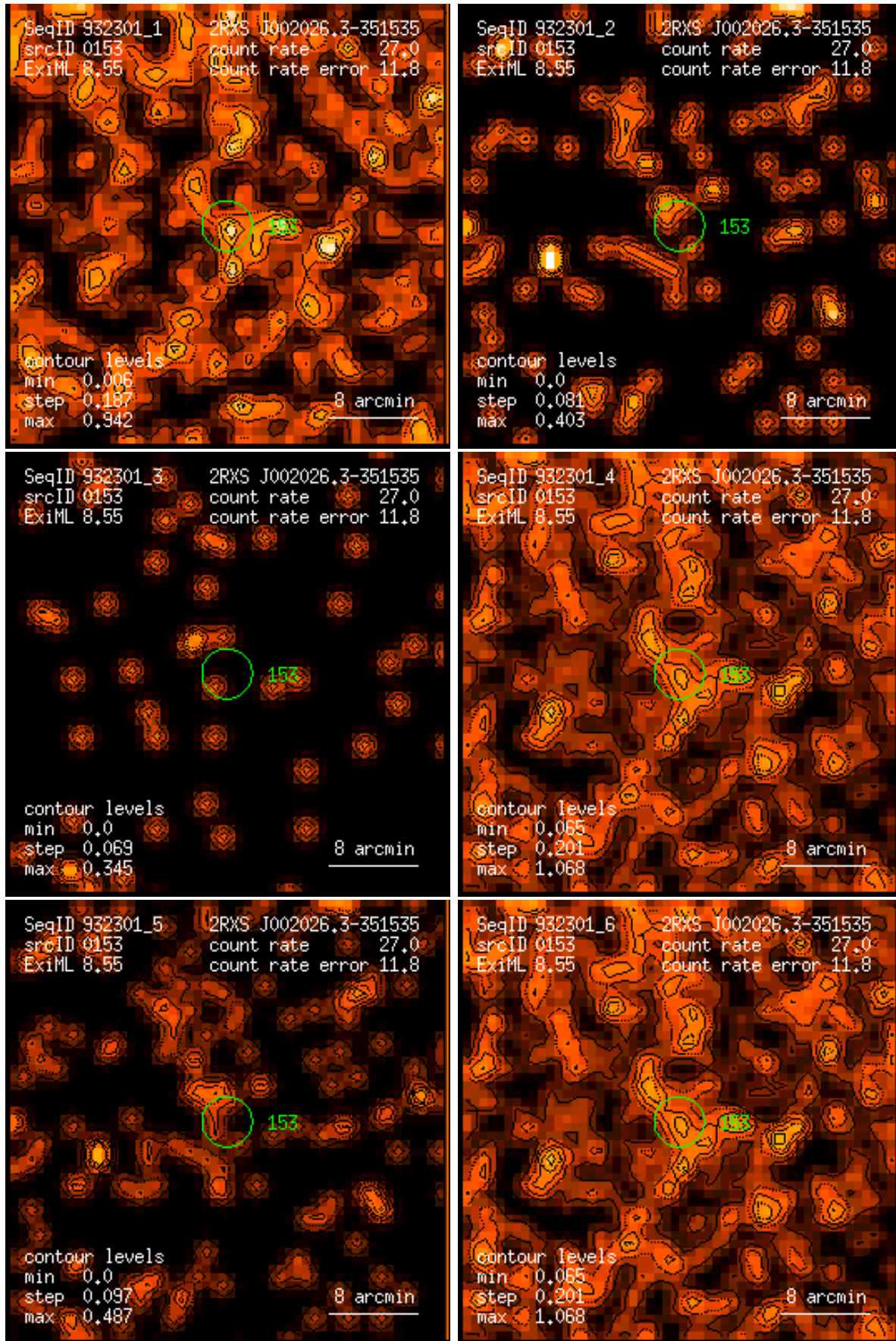
Figure 153: RASS 932301: detection 0153: band rate images, Gaussian filter: (1) PSPC channels 11 – 41, (2) 52 – 90, (3) 91 – 201, (4) 11 – 235, (5) 52 – 201, (6) 11 – 201. Broad band rates in counts/ks. Band rate contour levels in counts/ks/arcmin 2 .
