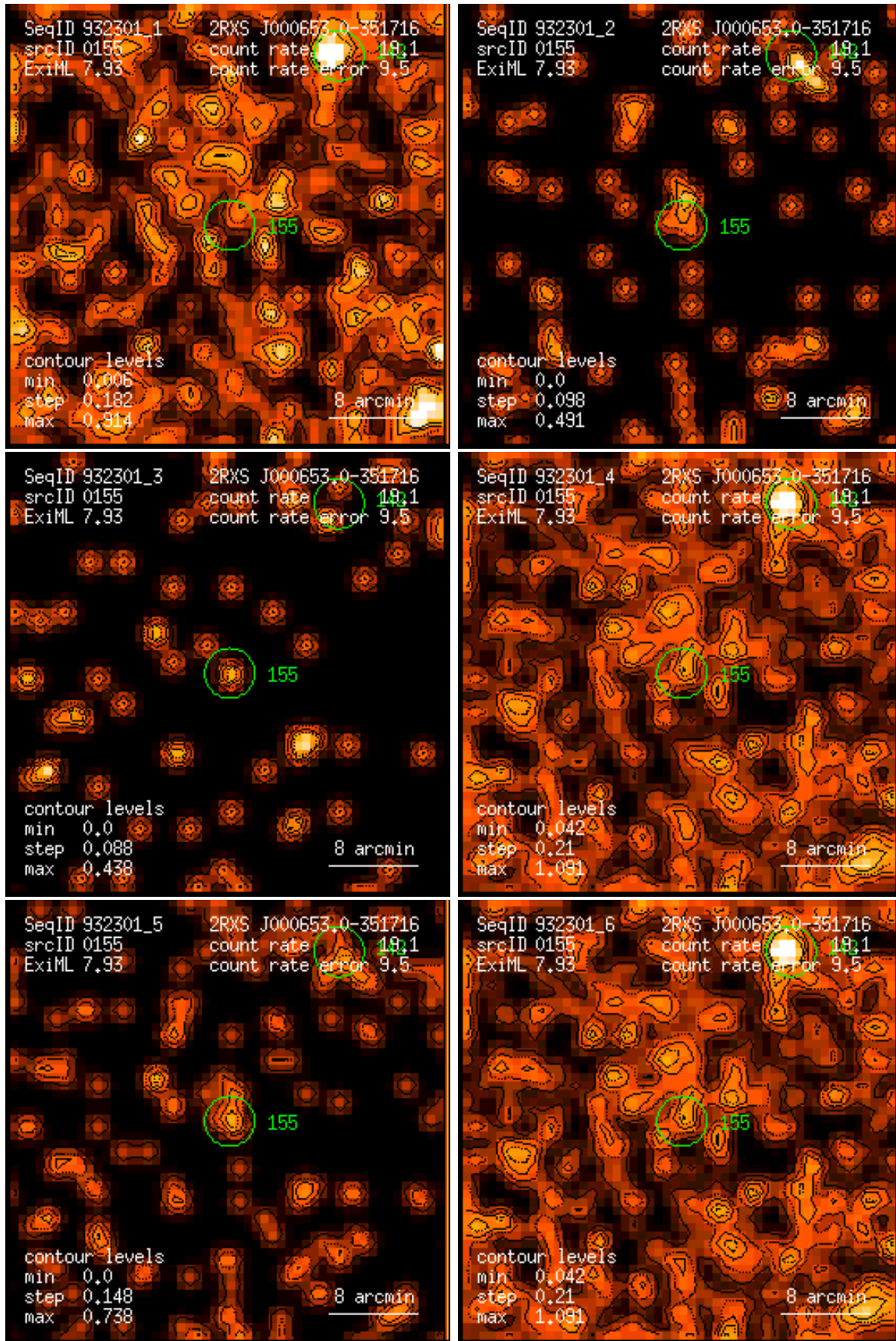
Figure 155: RASS 932301: detection 0155: band rate images, Gaussian filter: (1) PSPC channels 11 – 41, (2) 52 – 90, (3) 91 – 201, (4) 11 – 235, (5) 52 – 201, (6) 11 – 201. Broad band rates in counts/ks. Band rate contour levels in counts/ks/arcmin 2 .
