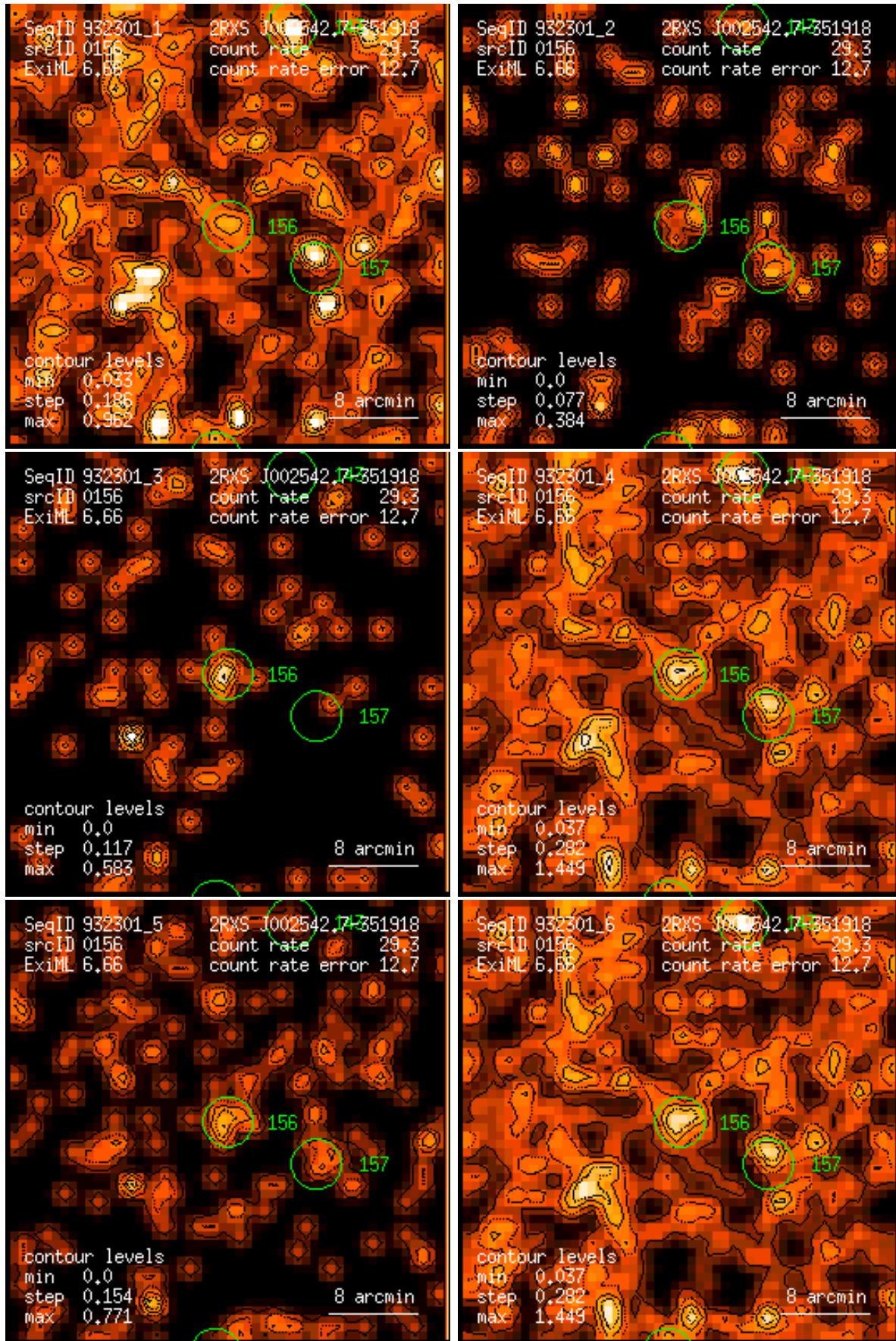
Figure 156: RASS 932301: detection 0156: band rate images, Gaussian filter: (1) PSPC channels 11 – 41, (2) 52 – 90, (3) 91 – 201, (4) 11 – 235, (5) 52 – 201, (6) 11 – 201. Broad band rates in counts/ks. Band rate contour levels in counts/ks/arcmin 2 .
