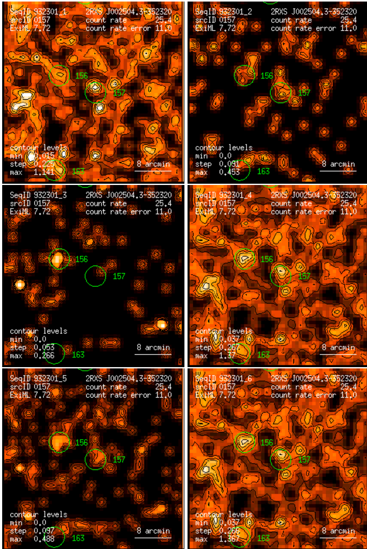
Figure 157: RASS 932301: detection 0157: band rate images, Gaussian filter: (1) PSPC channels 11 – 41, (2) 52 – 90, (3) 91 – 201, (4) 11 – 235, (5) 52 – 201, (6) 11 – 201. Broad band rates in counts/ks. Band rate contour levels in counts/ks/arcmin 2 .
