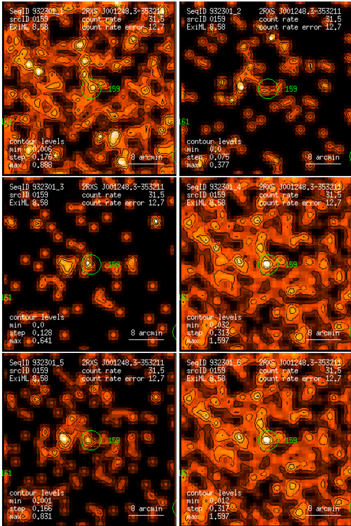
Figure 159: RASS 932301: detection 0159: band rate images, Gaussian filter: (1) PSPC channels 11 – 41, (2) 52 – 90, (3) 91 – 201, (4) 11 – 235, (5) 52 – 201, (6) 11 – 201. Broad band rates in counts/ks. Band rate contour levels in counts/ks/arcmin 2 .
