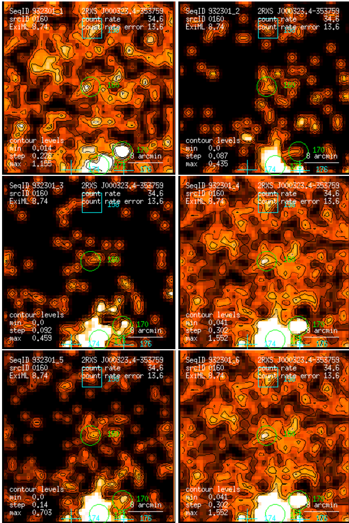
Figure 160: RASS 932301: detection 0160: band rate images, Gaussian filter: (1) PSPC channels 11 – 41, (2) 52 – 90, (3) 91 – 201, (4) 11 – 235, (5) 52 – 201, (6) 11 – 201. Broad band rates in counts/ks. Band rate contour levels in counts/ks/arcmin 2 .
