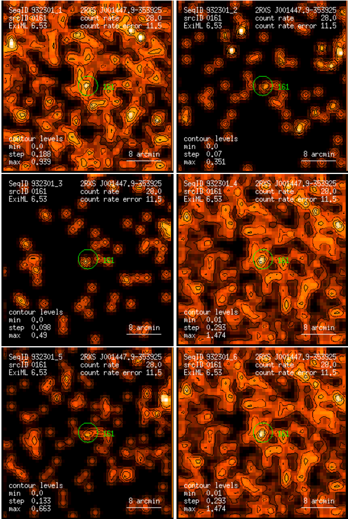
Figure 161: RASS 932301: detection 0161: band rate images, Gaussian filter: (1) PSPC channels 11 – 41, (2) 52 – 90, (3) 91 – 201, (4) 11 – 235, (5) 52 – 201, (6) 11 – 201. Broad band rates in counts/ks. Band rate contour levels in counts/ks/arcmin 2 .
