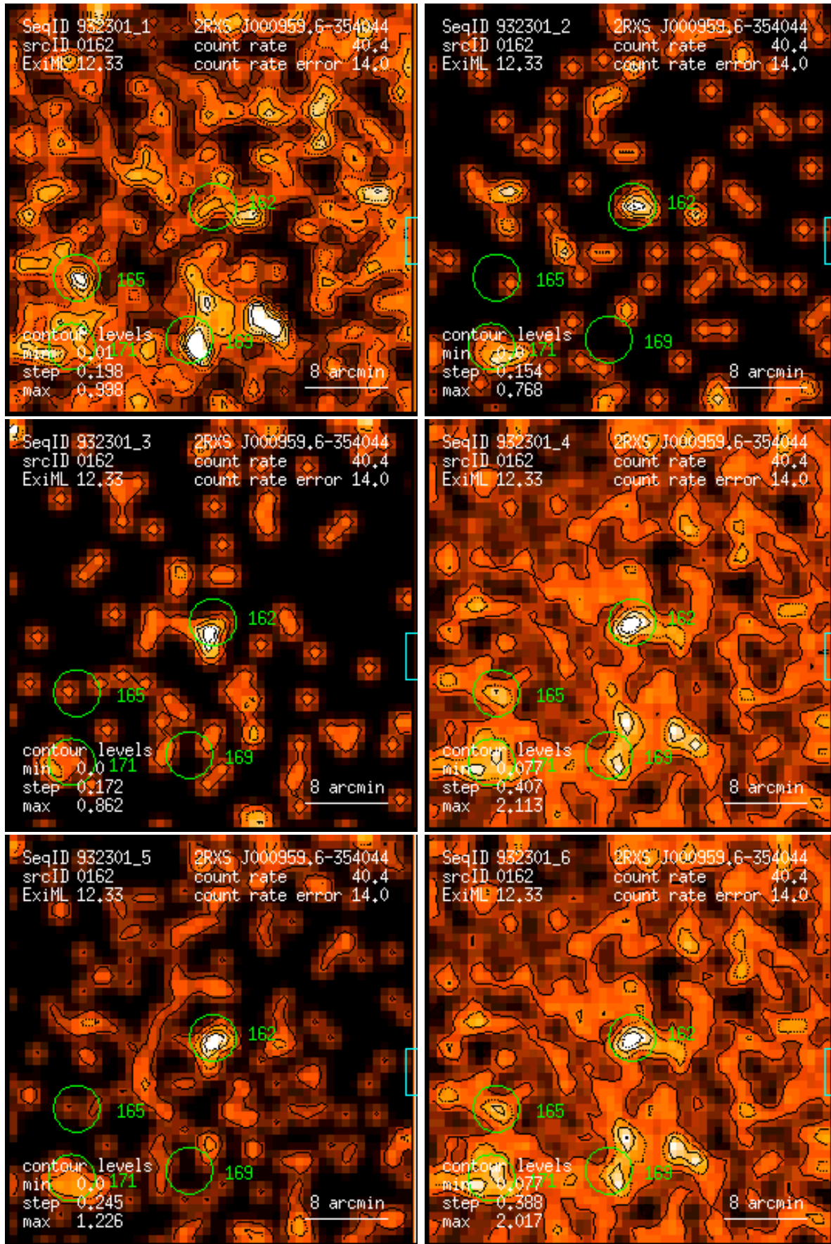
Figure 162: RASS 932301: detection 0162: band rate images, Gaussian filter: (1) PSPC channels 11 – 41, (2) 52 – 90, (3) 91 – 201, (4) 11 – 235, (5) 52 – 201, (6) 11 – 201. Broad band rates in counts/ks. Band rate contour levels in counts/ks/arcmin 2 .
