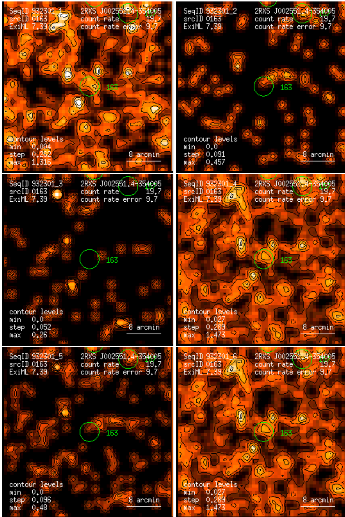
Figure 163: RASS 932301: detection 0163: band rate images, Gaussian filter: (1) PSPC channels 11 – 41, (2) 52 – 90, (3) 91 – 201, (4) 11 – 235, (5) 52 – 201, (6) 11 – 201. Broad band rates in counts/ks. Band rate contour levels in counts/ks/arcmin 2 .
