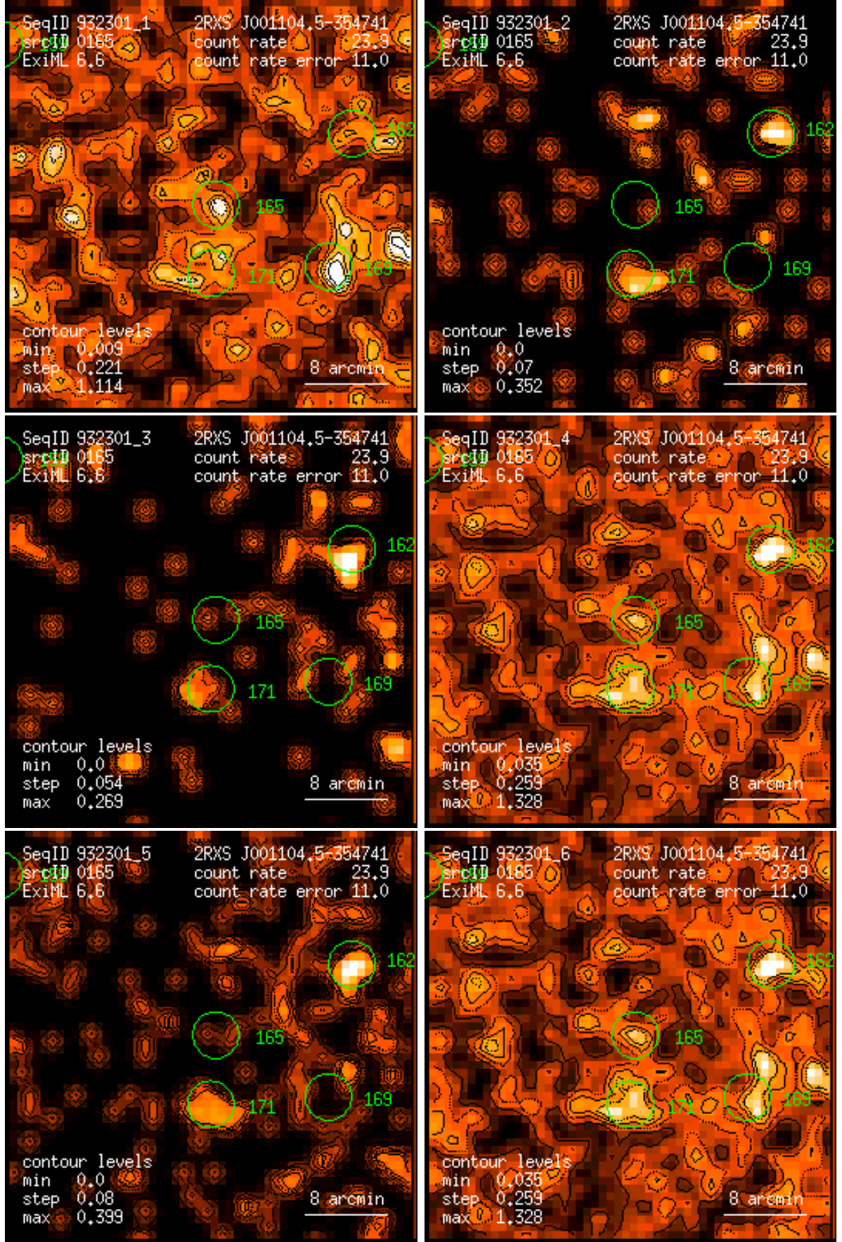
Figure 165: RASS 932301: detection 0165: band rate images, Gaussian filter: (1) PSPC channels 11 – 41, (2) 52 – 90, (3) 91 – 201, (4) 11 – 235, (5) 52 – 201, (6) 11 – 201. Broad band rates in counts/ks. Band rate contour levels in counts/ks/arcmin 2 .
