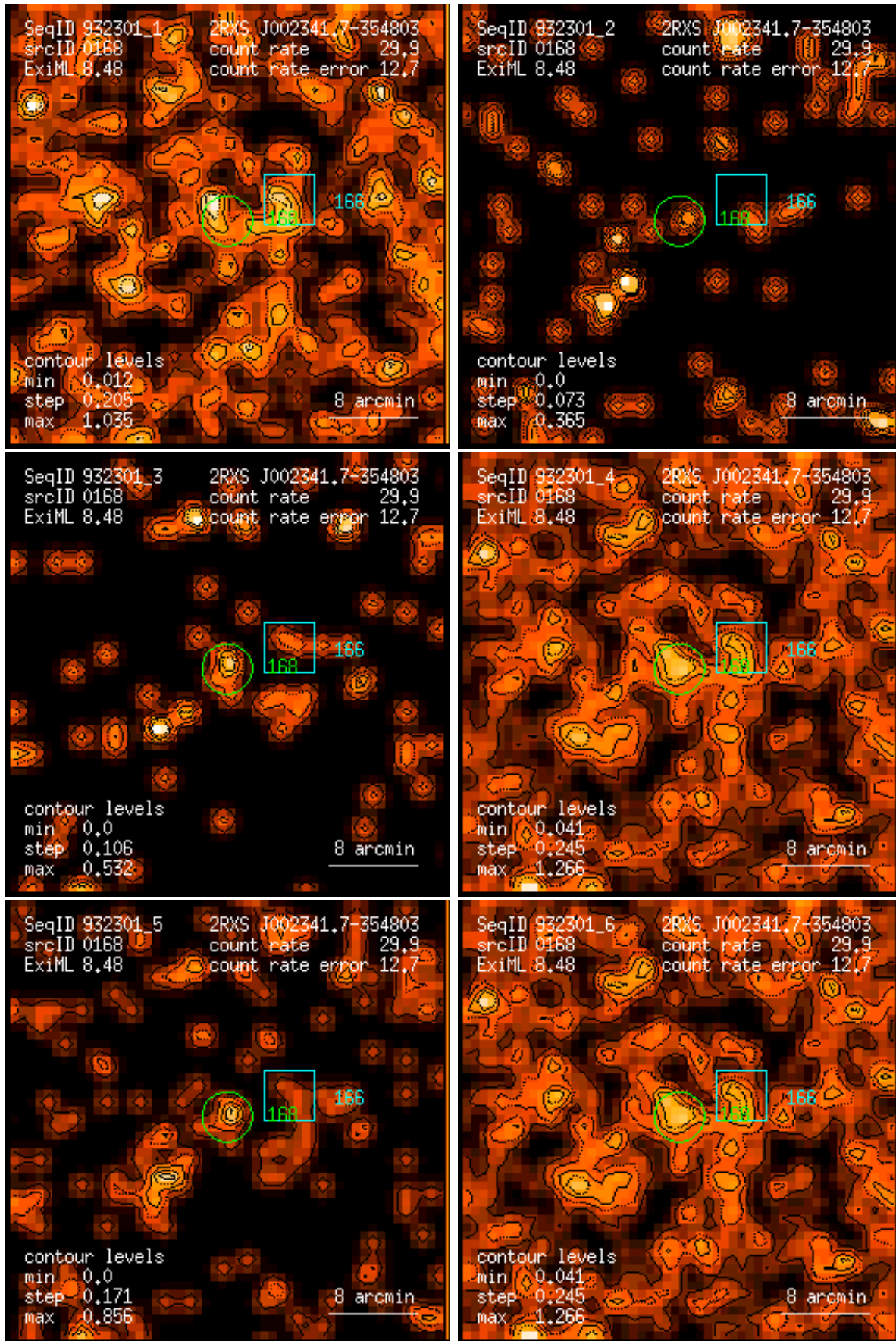
Figure 168: RASS 932301: detection 0168: band rate images, Gaussian filter: (1) PSPC channels 11 – 41, (2) 52 – 90, (3) 91 – 201, (4) 11 – 235, (5) 52 – 201, (6) 11 – 201. Broad band rates in counts/ks. Band rate contour levels in counts/ks/arcmin 2 .
