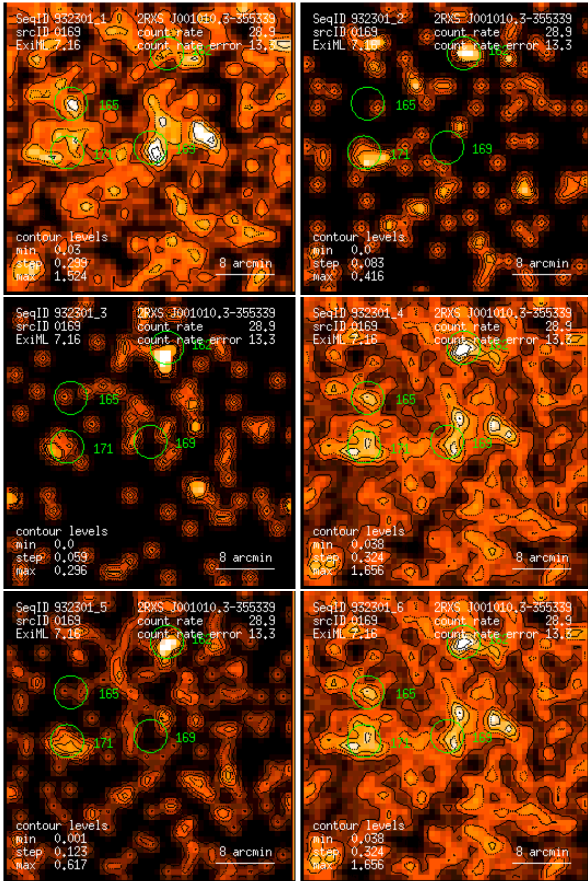
Figure 169: RASS 932301: detection 0169: band rate images, Gaussian filter: (1) PSPC channels 11 – 41, (2) 52 – 90, (3) 91 – 201, (4) 11 – 235, (5) 52 – 201, (6) 11 – 201. Broad band rates in counts/ks. Band rate contour levels in counts/ks/arcmin 2 .
