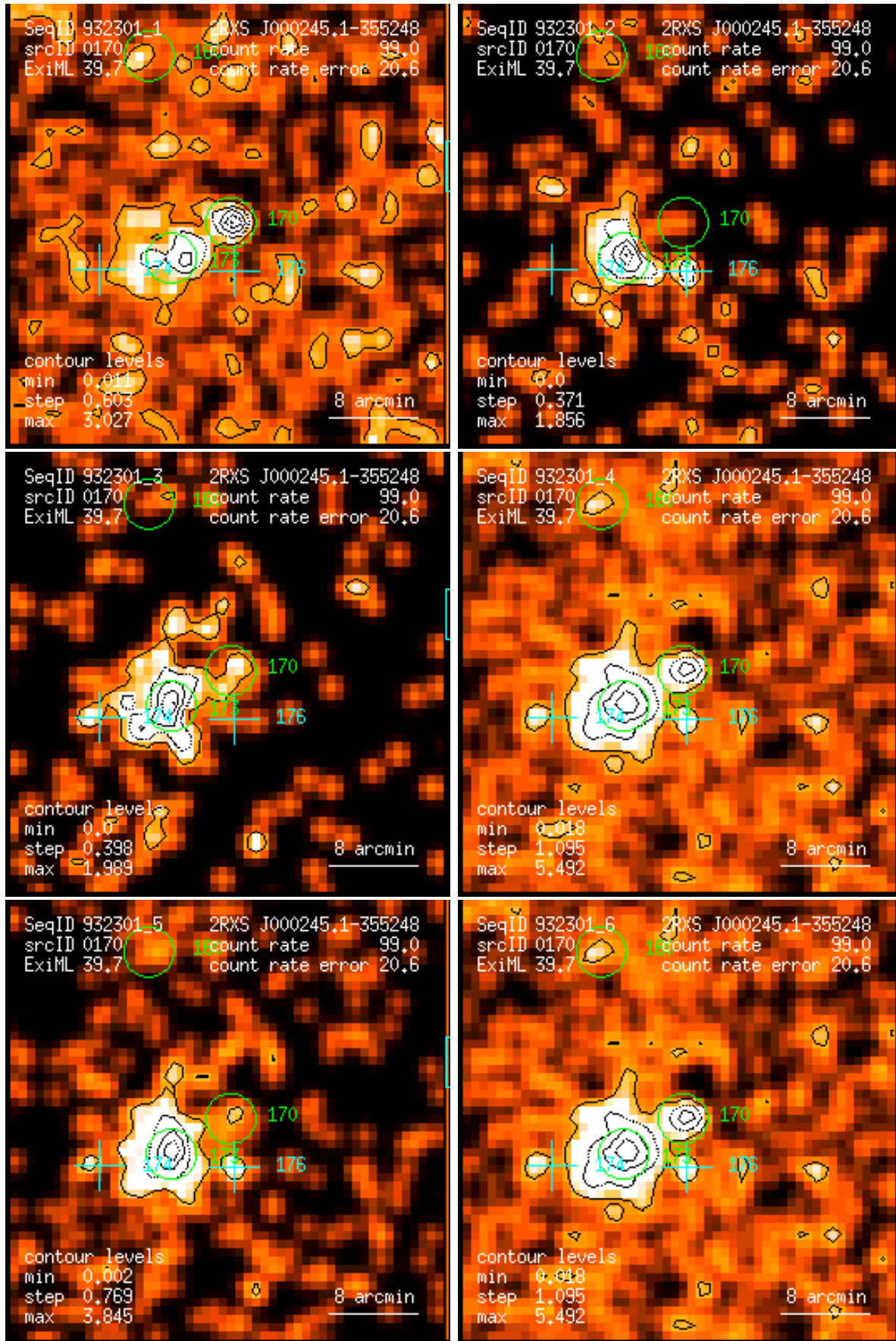
Figure 170: RASS 932301: detection 0170: band rate images, Gaussian filter: (1) PSPC channels 11 – 41, (2) 52 – 90, (3) 91 – 201, (4) 11 – 235, (5) 52 – 201, (6) 11 – 201. Broad band rates in counts/ks. Band rate contour levels in counts/ks/arcmin 2 .
