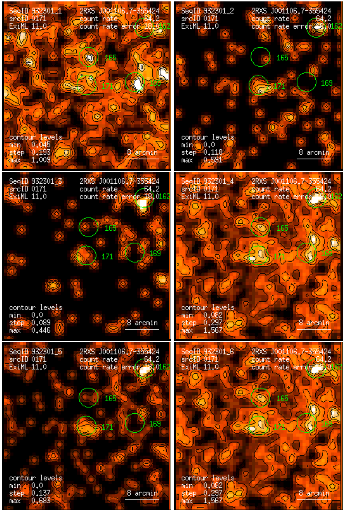
Figure 171: RASS 932301: detection 0171: band rate images, Gaussian filter: (1) PSPC channels 11 – 41, (2) 52 – 90, (3) 91 – 201, (4) 11 – 235, (5) 52 – 201, (6) 11 – 201. Broad band rates in counts/ks. Band rate contour levels in counts/ks/arcmin 2 .
