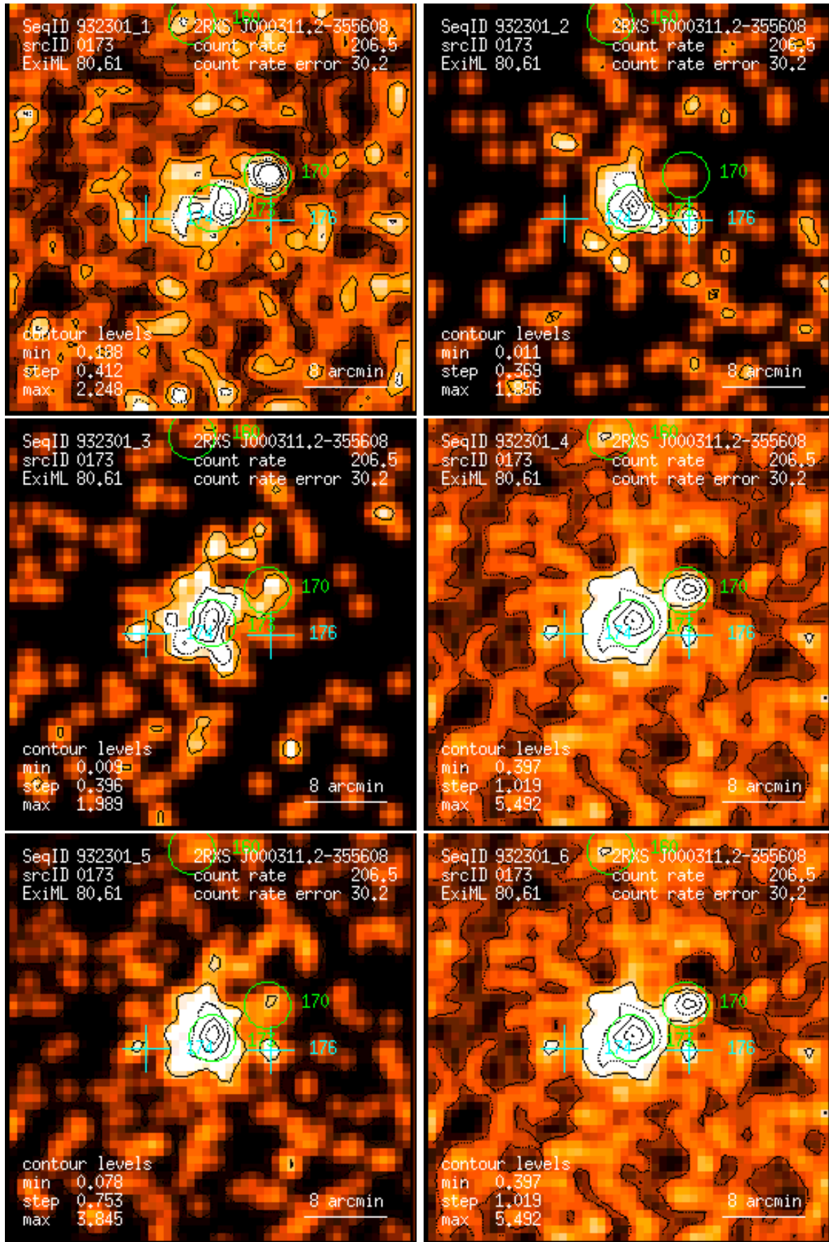
Figure 173: RASS 932301: detection 0173: band rate images, Gaussian filter: (1) PSPC channels 11 – 41, (2) 52 – 90, (3) 91 – 201, (4) 11 – 235, (5) 52 – 201, (6) 11 – 201. Broad band rates in counts/ks. Band rate contour levels in counts/ks/arcmin 2 .
