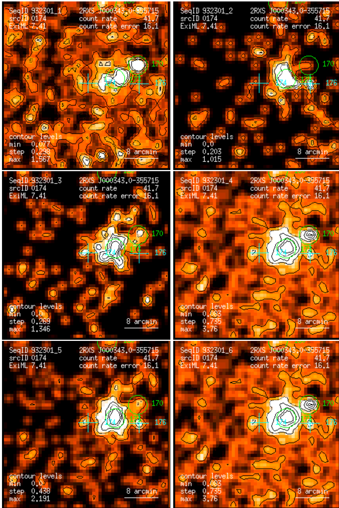
Figure 174: RASS 932301: detection 0174: band rate images, Gaussian filter: (1) PSPC channels 11 – 41, (2) 52 – 90, (3) 91 – 201, (4) 11 – 235, (5) 52 – 201, (6) 11 – 201. Broad band rates in counts/ks. Band rate contour levels in counts/ks/arcmin 2 .
