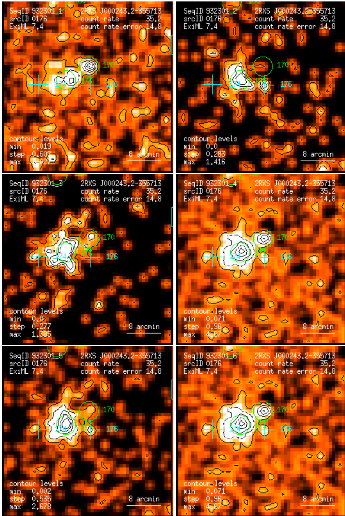
Figure 176: RASS 932301: detection 0176: band rate images, Gaussian filter: (1) PSPC channels 11 – 41, (2) 52 – 90, (3) 91 – 201, (4) 11 – 235, (5) 52 – 201, (6) 11 – 201. Broad band rates in counts/ks. Band rate contour levels in counts/ks/arcmin 2 .
