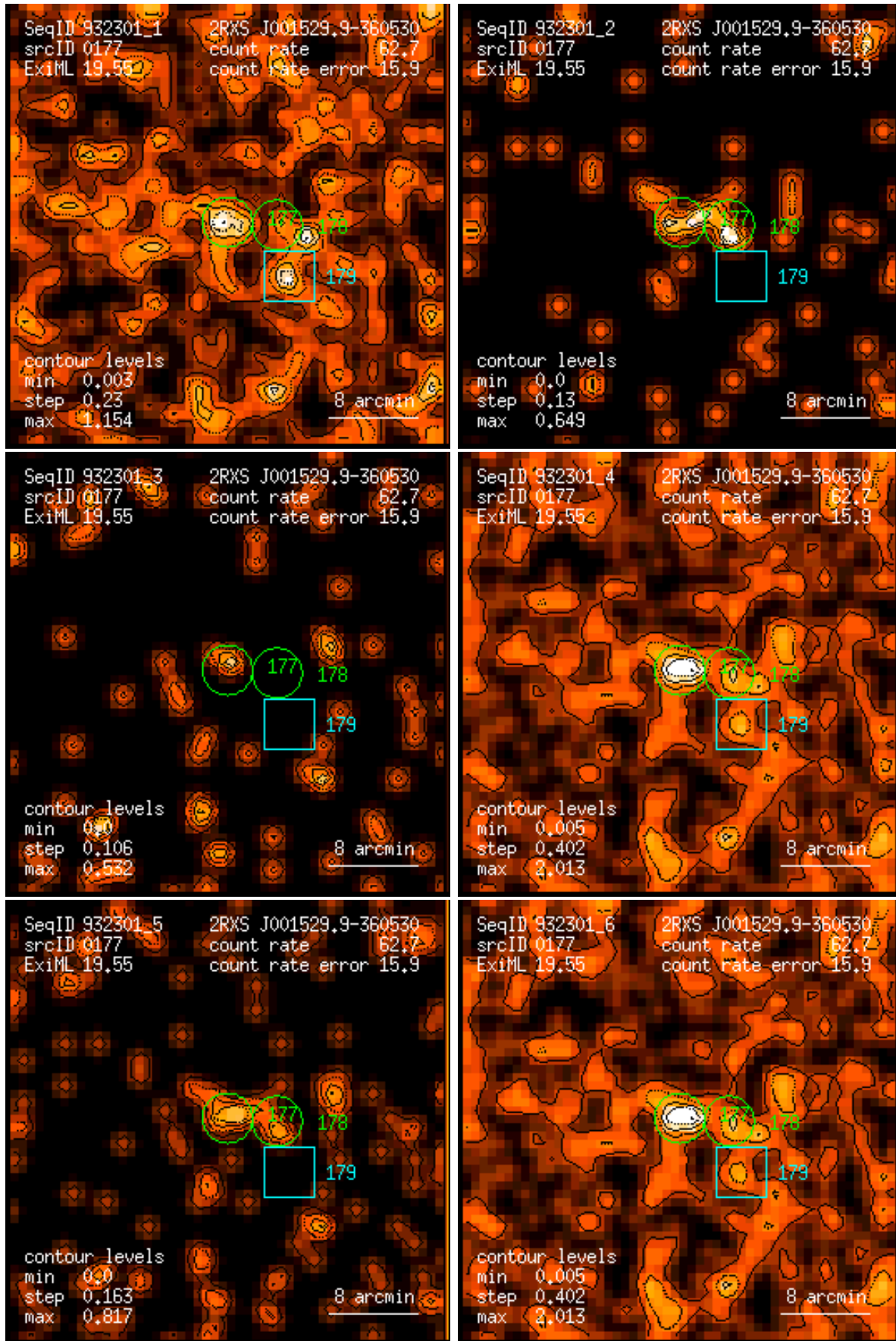
Figure 177: RASS 932301: detection 0177: band rate images, Gaussian filter: (1) PSPC channels 11 – 41, (2) 52 – 90, (3) 91 – 201, (4) 11 – 235, (5) 52 – 201, (6) 11 – 201. Broad band rates in counts/ks. Band rate contour levels in counts/ks/arcmin 2 .
