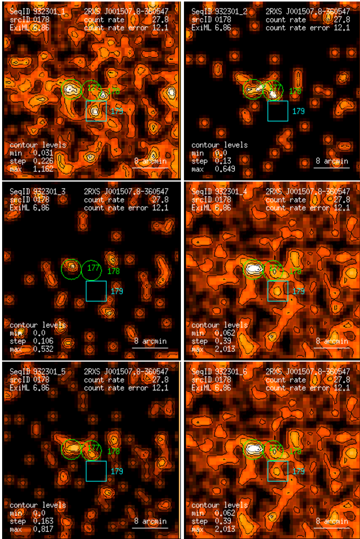
Figure 178: RASS 932301: detection 0178: band rate images, Gaussian filter: (1) PSPC channels 11 – 41, (2) 52 – 90, (3) 91 – 201, (4) 11 – 235, (5) 52 – 201, (6) 11 – 201. Broad band rates in counts/ks. Band rate contour levels in counts/ks/arcmin 2 .
