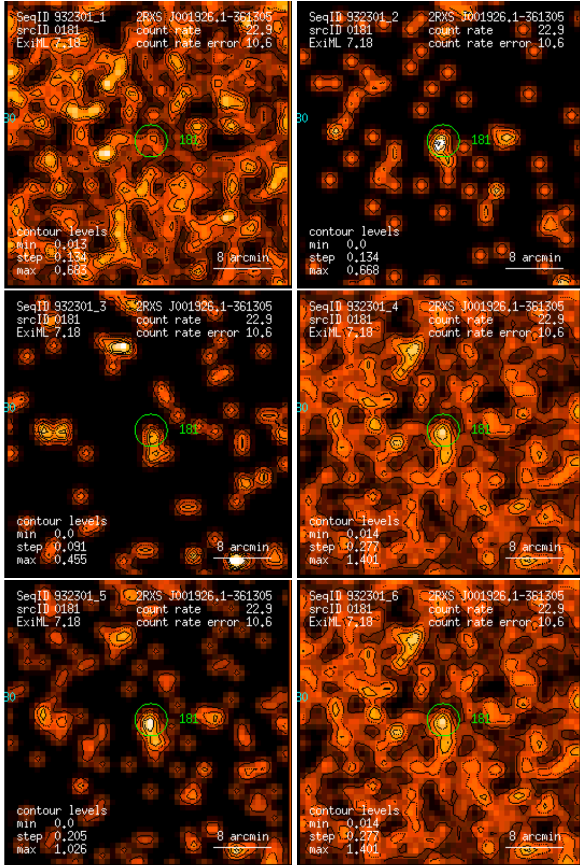
Figure 181: RASS 932301: detection 0181: band rate images, Gaussian filter: (1) PSPC channels 11 – 41, (2) 52 – 90, (3) 91 – 201, (4) 11 – 235, (5) 52 – 201, (6) 11 – 201. Broad band rates in counts/ks. Band rate contour levels in counts/ks/arcmin 2 .
