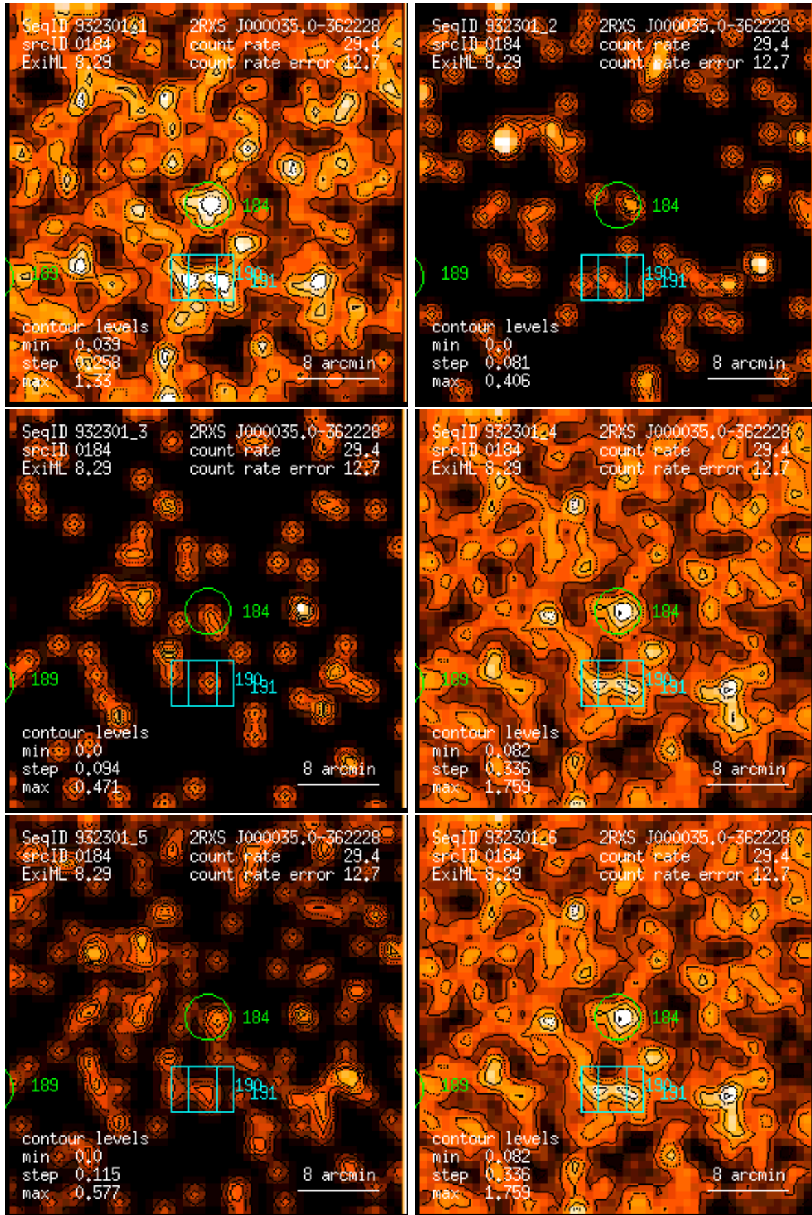
Figure 184: RASS 932301: detection 0184: band rate images, Gaussian filter: (1) PSPC channels 11 – 41, (2) 52 – 90, (3) 91 – 201, (4) 11 – 235, (5) 52 – 201, (6) 11 – 201. Broad band rates in counts/ks. Band rate contour levels in counts/ks/arcmin 2 .
