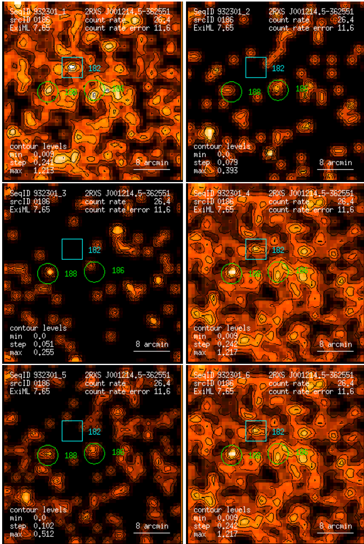
Figure 186: RASS 932301: detection 0186: band rate images, Gaussian filter: (1) PSPC channels 11 – 41, (2) 52 – 90, (3) 91 – 201, (4) 11 – 235, (5) 52 – 201, (6) 11 – 201. Broad band rates in counts/ks. Band rate contour levels in counts/ks/arcmin 2 .
