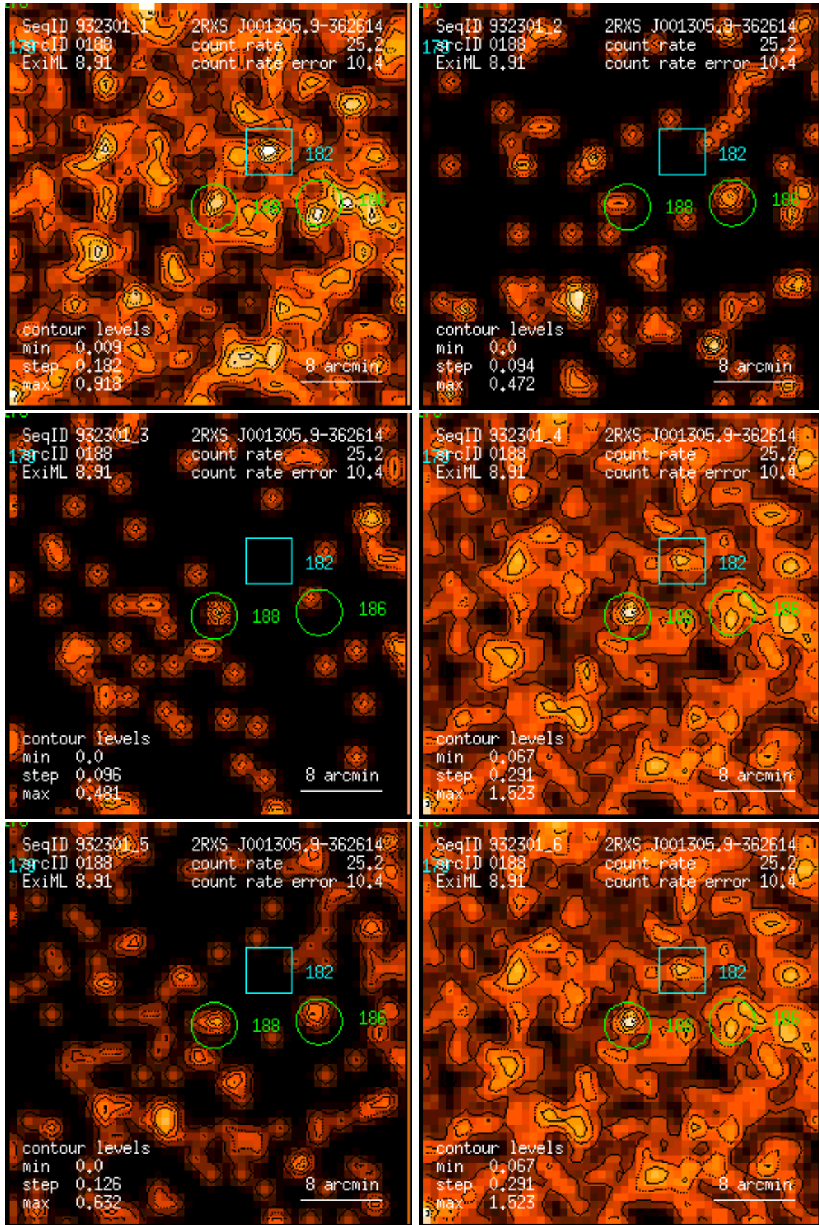
Figure 188: RASS 932301: detection 0188: band rate images, Gaussian filter: (1) PSPC channels 11 – 41, (2) 52 – 90, (3) 91 – 201, (4) 11 – 235, (5) 52 – 201, (6) 11 – 201. Broad band rates in counts/ks. Band rate contour levels in counts/ks/arcmin 2 .
