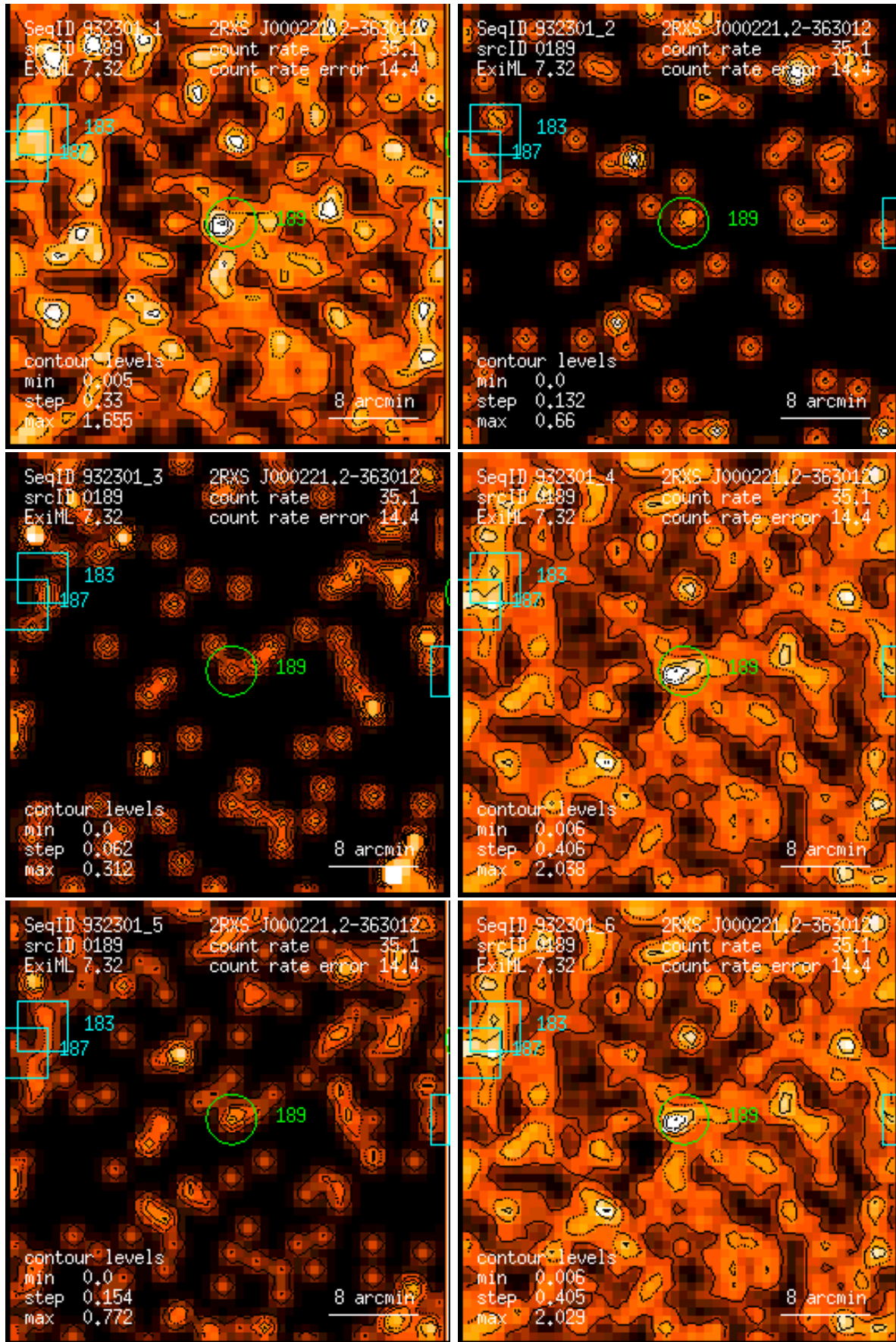
Figure 189: RASS 932301: detection 0189: band rate images, Gaussian filter: (1) PSPC channels 11 – 41, (2) 52 – 90, (3) 91 – 201, (4) 11 – 235, (5) 52 – 201, (6) 11 – 201. Broad band rates in counts/ks. Band rate contour levels in counts/ks/arcmin 2 .
