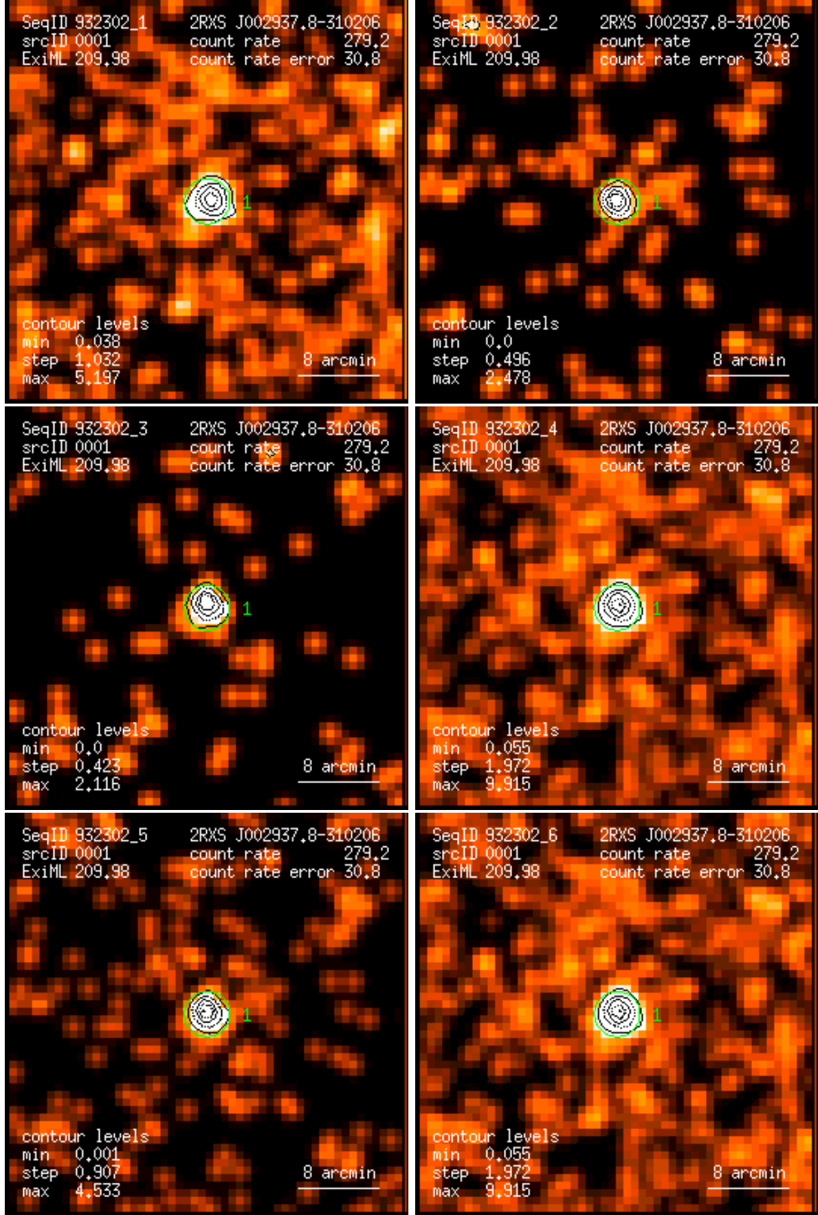
Figure 1: RASS 932302: detection 0001: band rate images, Gaussian filter: (1) PSPC channels 11 – 41, (2) 52 – 90, (3) 91 – 201, (4) 11 – 235, (5) 52 – 201, (6) 11 – 201. Broad band rates in counts/ks. Band rate contour levels in counts/ks/arcmin 2 .
