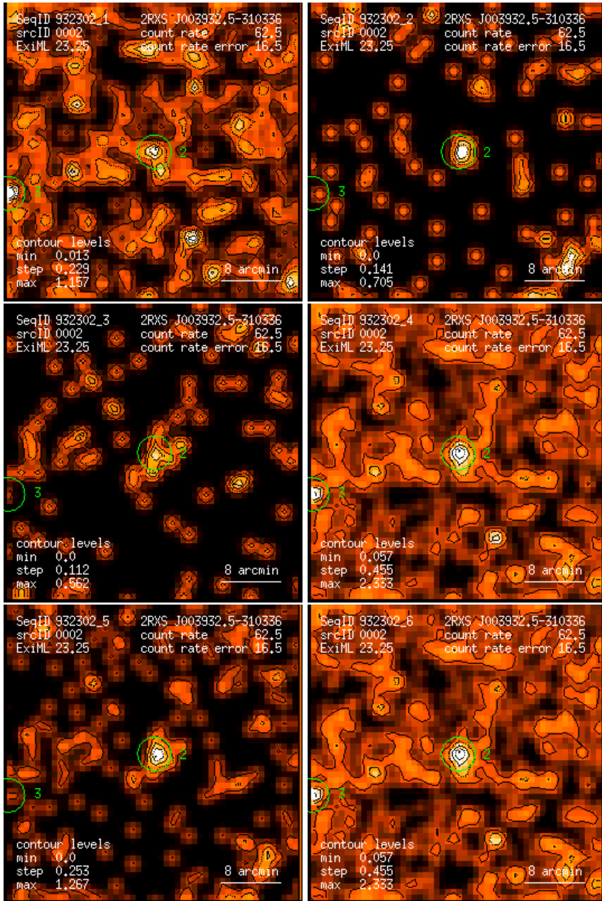
Figure 2: RASS 932302: detection 0002: band rate images, Gaussian filter: (1) PSPC channels 11 – 41, (2) 52 – 90, (3) 91 – 201, (4) 11 – 235, (5) 52 – 201, (6) 11 – 201. Broad band rates in counts/ks. Band rate contour levels in counts/ks/arcmin 2 .
