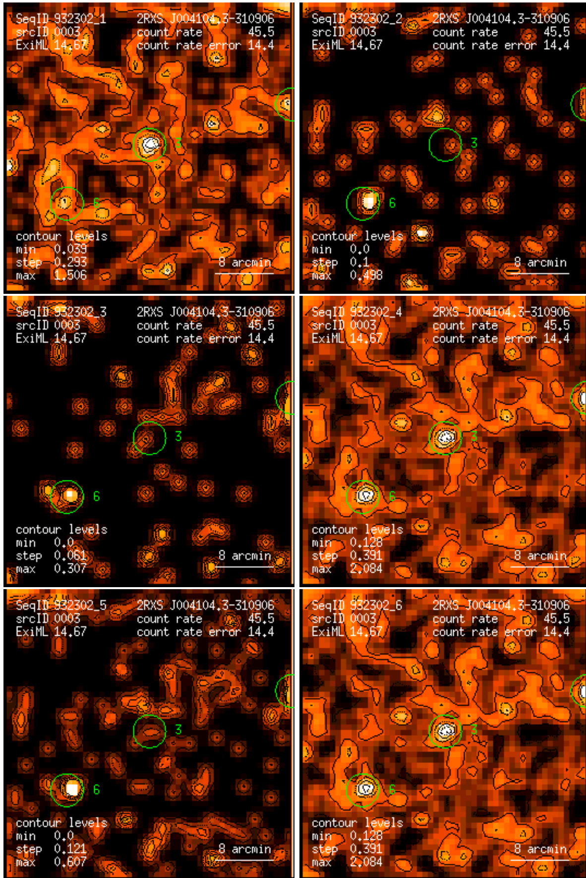
Figure 3: RASS 932302: detection 0003: band rate images, Gaussian filter: (1) PSPC channels 11 – 41, (2) 52 – 90, (3) 91 – 201, (4) 11 – 235, (5) 52 – 201, (6) 11 – 201. Broad band rates in counts/ks. Band rate contour levels in counts/ks/arcmin 2 .
