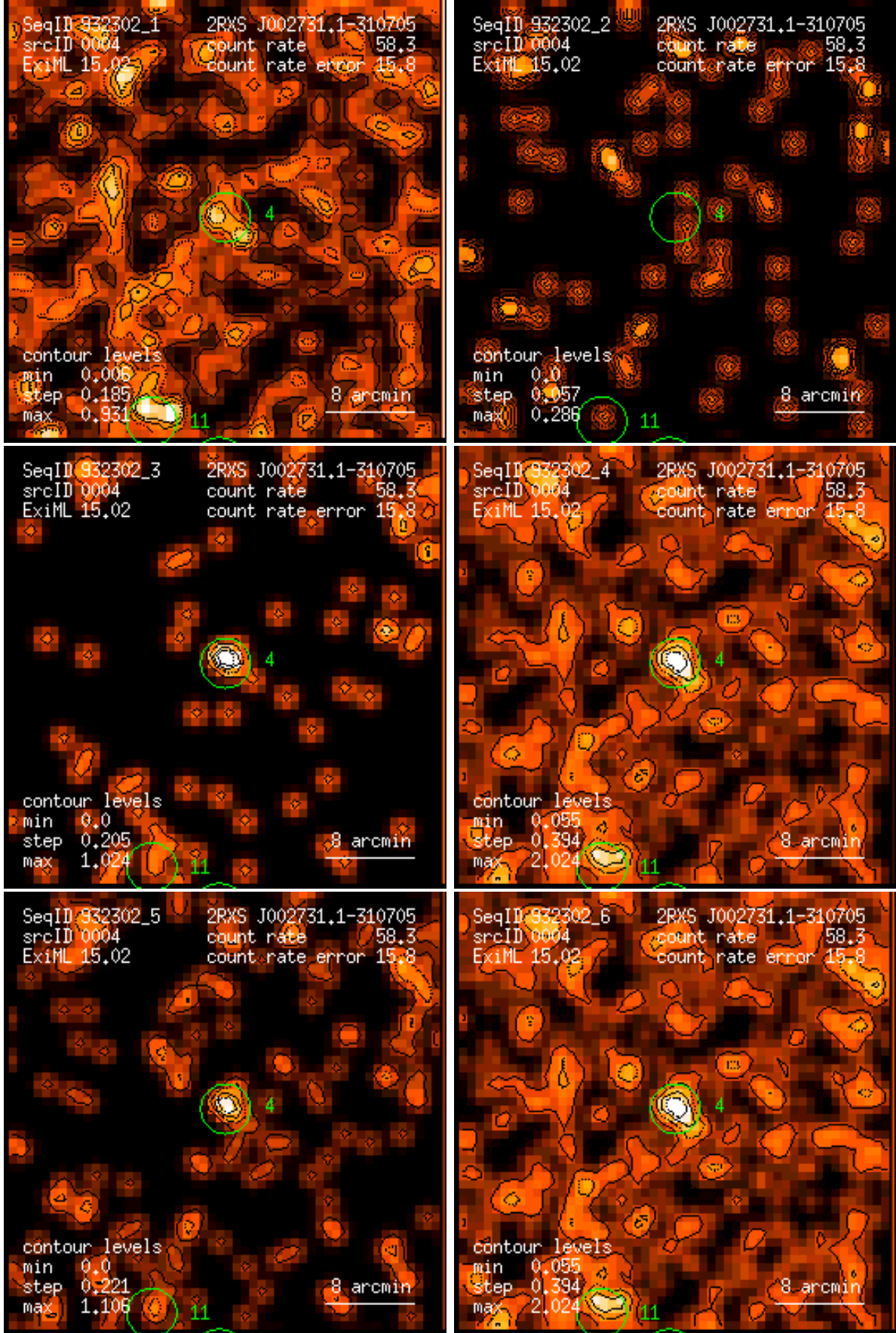
Figure 4: RASS 932302: detection 0004: band rate images, Gaussian filter: (1) PSPC channels 11 – 41, (2) 52 – 90, (3) 91 – 201, (4) 11 – 235, (5) 52 – 201, (6) 11 – 201. Broad band rates in counts/ks. Band rate contour levels in counts/ks/arcmin 2 .
