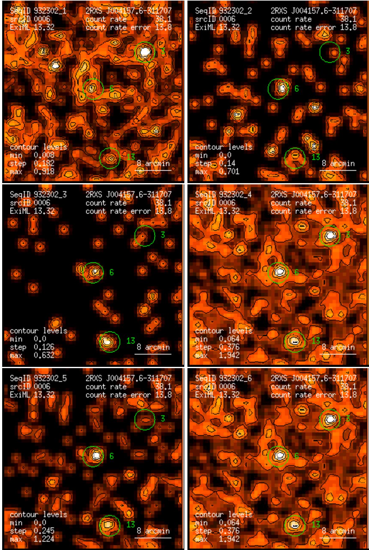
Figure 6: RASS 932302: detection 0006: band rate images, Gaussian filter: (1) PSPC channels 11 – 41, (2) 52 – 90, (3) 91 – 201, (4) 11 – 235, (5) 52 – 201, (6) 11 – 201. Broad band rates in counts/ks. Band rate contour levels in counts/ks/arcmin 2 .
