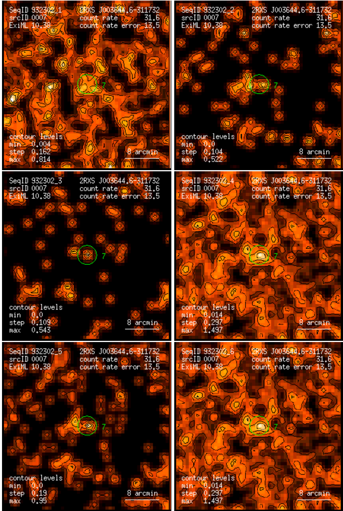
Figure 7: RASS 932302: detection 0007: band rate images, Gaussian filter: (1) PSPC channels 11 – 41, (2) 52 – 90, (3) 91 – 201, (4) 11 – 235, (5) 52 – 201, (6) 11 – 201. Broad band rates in counts/ks. Band rate contour levels in counts/ks/arcmin 2 .
