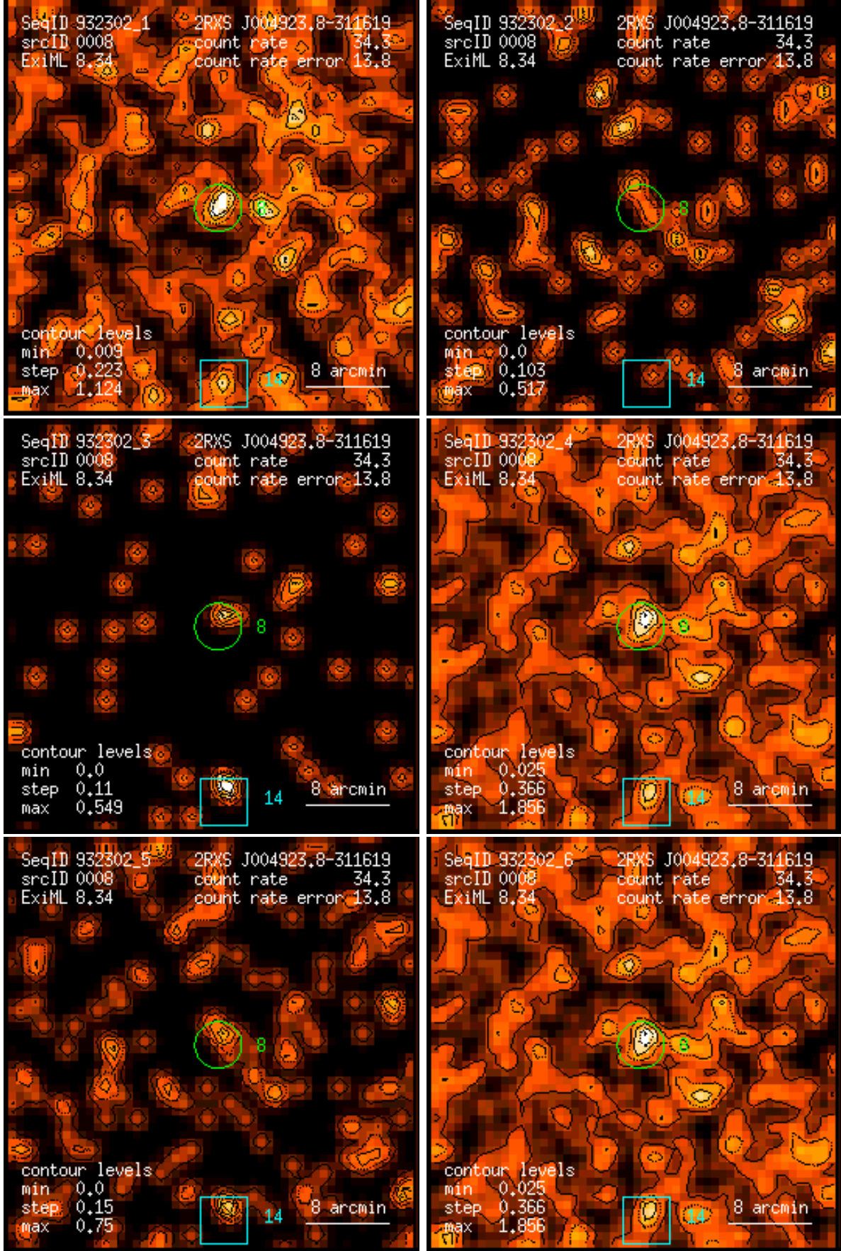
Figure 8: RASS 932302: detection 0008: band rate images, Gaussian filter: (1) PSPC channels 11 – 41, (2) 52 – 90, (3) 91 – 201, (4) 11 – 235, (5) 52 – 201, (6) 11 – 201. Broad band rates in counts/ks. Band rate contour levels in counts/ks/arcmin 2 .
