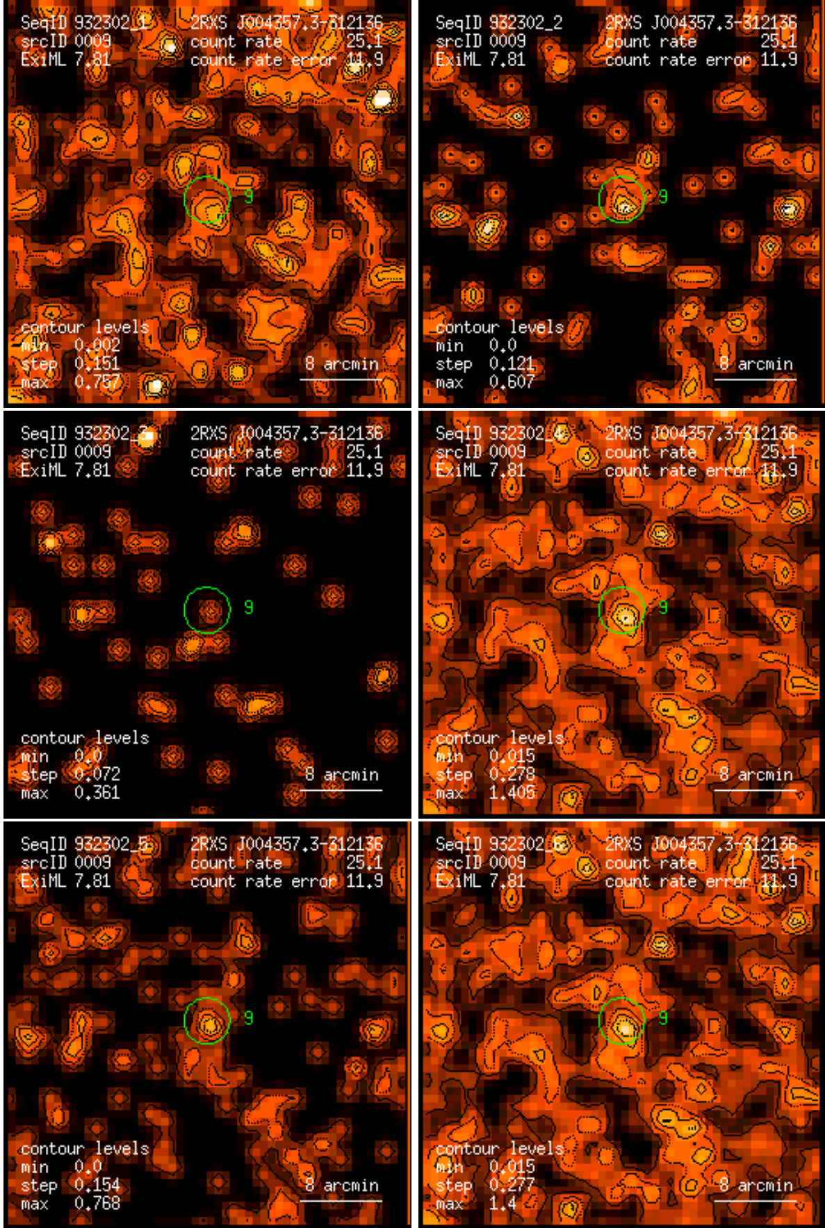
Figure 9: RASS 932302: detection 0009: band rate images, Gaussian filter: (1) PSPC channels 11 – 41, (2) 52 – 90, (3) 91 – 201, (4) 11 – 235, (5) 52 – 201, (6) 11 – 201. Broad band rates in counts/ks. Band rate contour levels in counts/ks/arcmin 2 .
