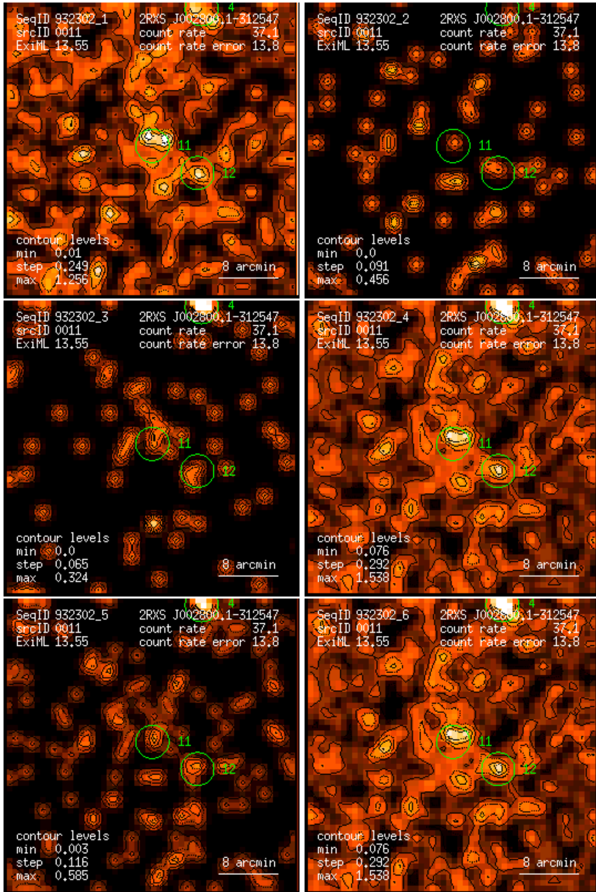
Figure 11: RASS 932302: detection 0011: band rate images, Gaussian filter: (1) PSPC channels 11 – 41, (2) 52 – 90, (3) 91 – 201, (4) 11 – 235, (5) 52 – 201, (6) 11 – 201. Broad band rates in counts/ks. Band rate contour levels in counts/ks/arcmin 2 .
