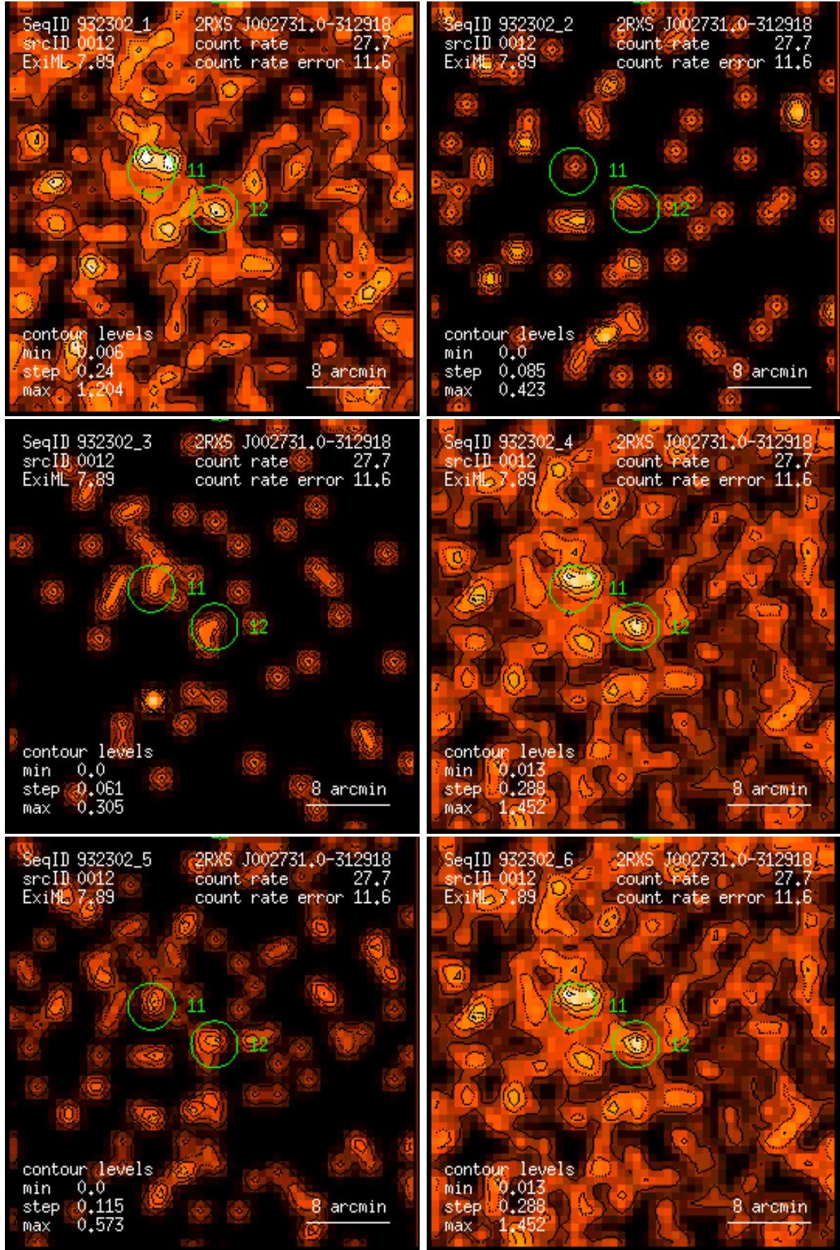
Figure 12: RASS 932302: detection 0012: band rate images, Gaussian filter: (1) PSPC channels 11 – 41, (2) 52 – 90, (3) 91 – 201, (4) 11 – 235, (5) 52 – 201, (6) 11 – 201. Broad band rates in counts/ks. Band rate contour levels in counts/ks/arcmin 2 .
