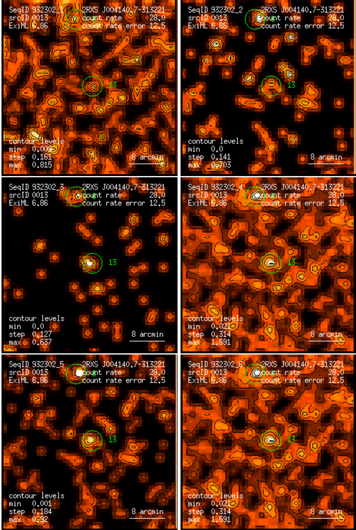
Figure 13: RASS 932302: detection 0013: band rate images, Gaussian filter: (1) PSPC channels 11 – 41, (2) 52 – 90, (3) 91 – 201, (4) 11 – 235, (5) 52 – 201, (6) 11 – 201. Broad band rates in counts/ks. Band rate contour levels in counts/ks/arcmin 2 .
